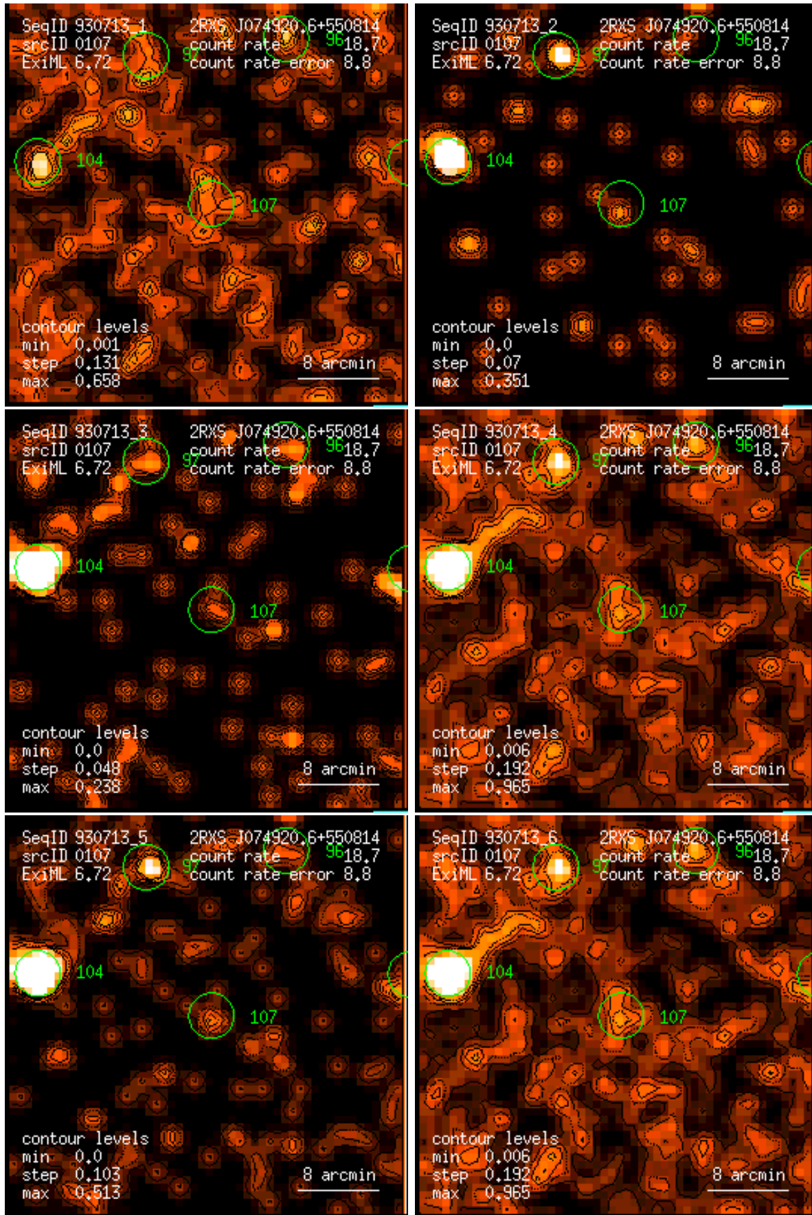
Figure 107: RASS 930713: detection 0107: band rate images, Gaussian filter: (1) PSPC channels 11 – 41, (2) 52 – 90, (3) 91 – 201, (4) 11 – 235, (5) 52 – 201, (6) 11 – 201. Broad band rates in counts/ks. Band rate contour levels in counts/ks/arcmin 2 .
