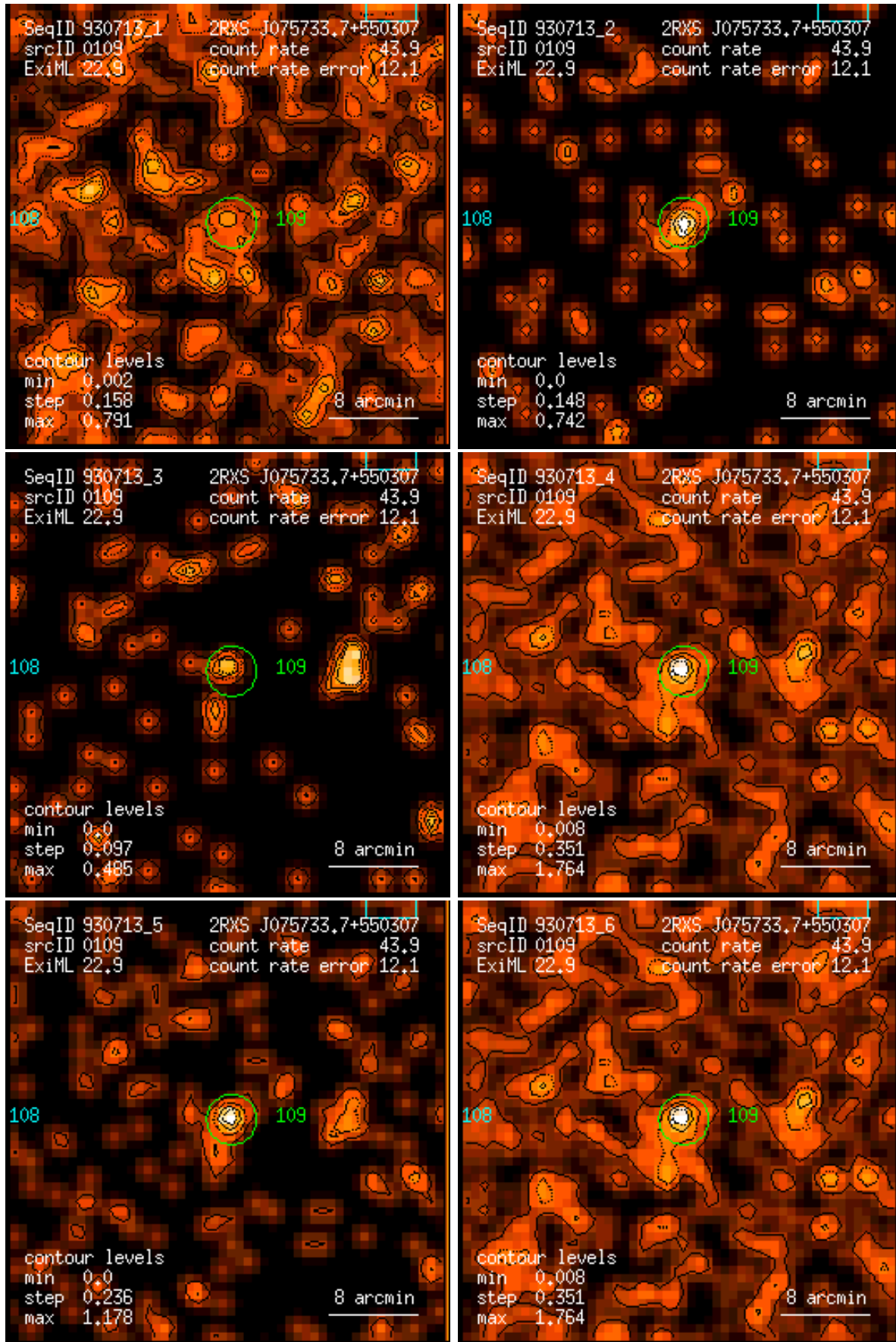
Figure 109: RASS 930713: detection 0109: band rate images, Gaussian filter: (1) PSPC channels 11 – 41, (2) 52 – 90, (3) 91 – 201, (4) 11 – 235, (5) 52 – 201, (6) 11 – 201. Broad band rates in counts/ks. Band rate contour levels in counts/ks/arcmin 2 .
