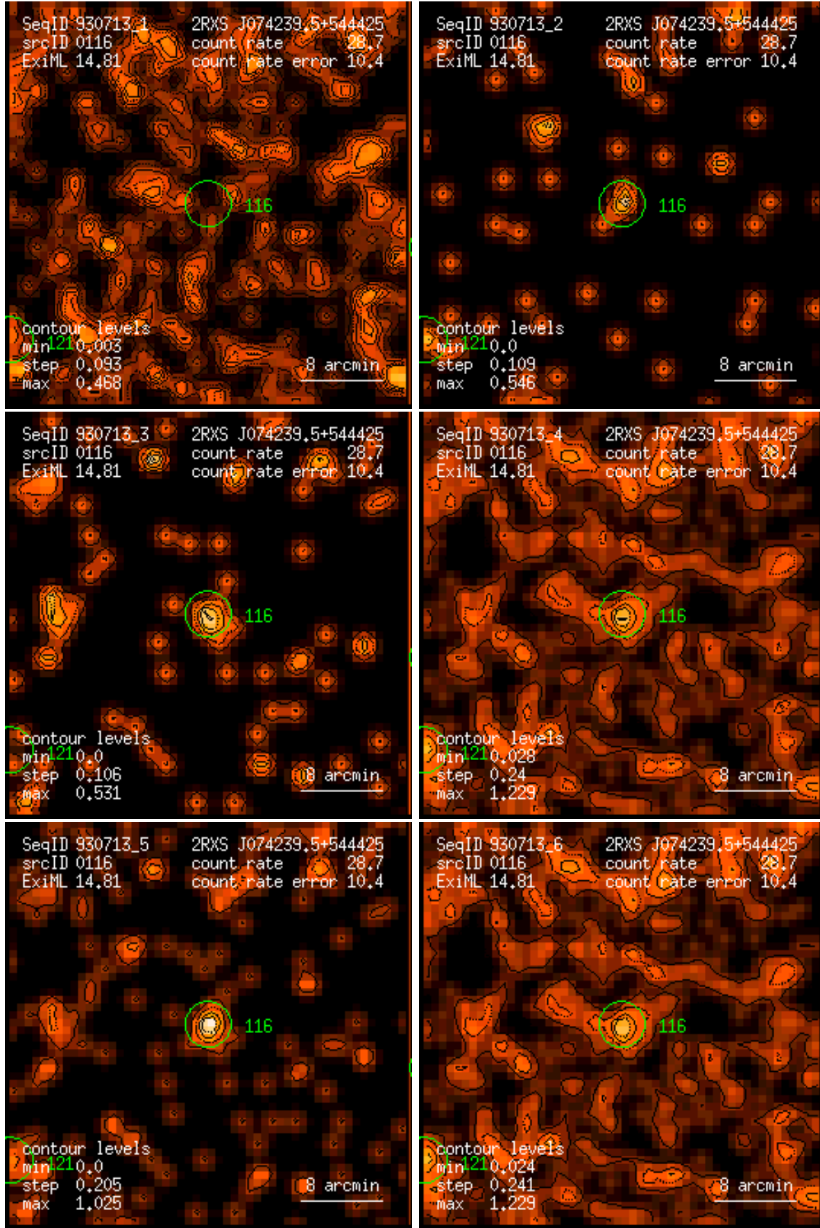
Figure 116: RASS 930713: detection 0116: band rate images, Gaussian filter: (1) PSPC channels 11 – 41, (2) 52 – 90, (3) 91 – 201, (4) 11 – 235, (5) 52 – 201, (6) 11 – 201. Broad band rates in counts/ks. Band rate contour levels in counts/ks/arcmin 2 .
