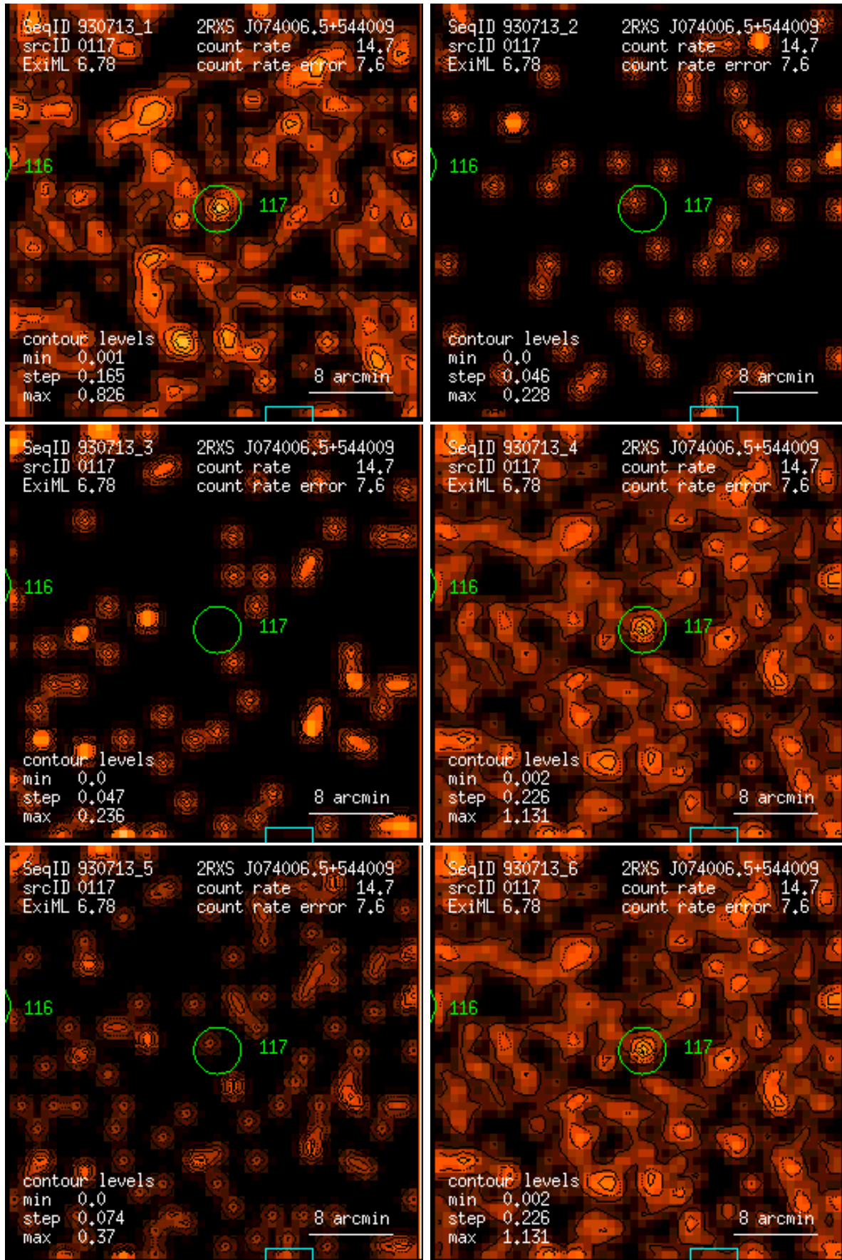
Figure 117: RASS 930713: detection 0117: band rate images, Gaussian filter: (1) PSPC channels 11 – 41, (2) 52 – 90, (3) 91 – 201, (4) 11 – 235, (5) 52 – 201, (6) 11 – 201. Broad band rates in counts/ks. Band rate contour levels in counts/ks/arcmin 2 .
