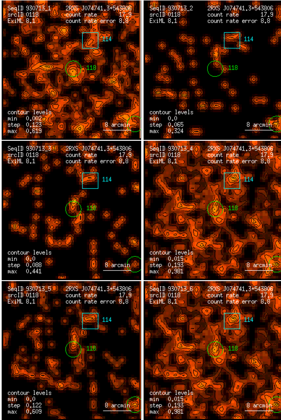
Figure 118: RASS 930713: detection 0118: band rate images, Gaussian filter: (1) PSPC channels 11 – 41, (2) 52 – 90, (3) 91 – 201, (4) 11 – 235, (5) 52 – 201, (6) 11 – 201. Broad band rates in counts/ks. Band rate contour levels in counts/ks/arcmin 2 .
