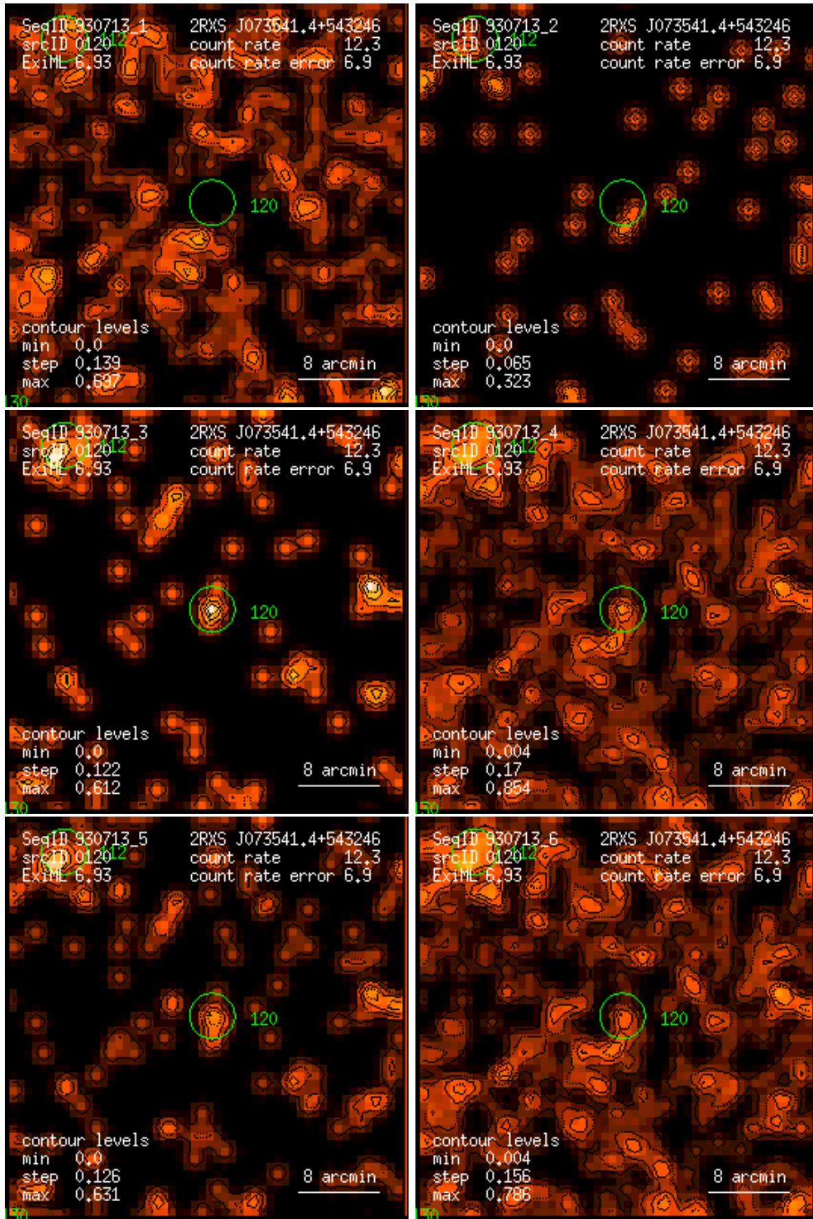
Figure 120: RASS 930713: detection 0120: band rate images, Gaussian filter: (1) PSPC channels 11 – 41, (2) 52 – 90, (3) 91 – 201, (4) 11 – 235, (5) 52 – 201, (6) 11 – 201. Broad band rates in counts/ks. Band rate contour levels in counts/ks/arcmin 2 .
