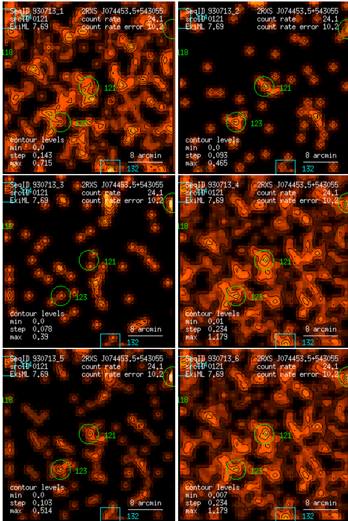
Figure 121: RASS 930713: detection 0121: band rate images, Gaussian filter: (1) PSPC channels 11 – 41, (2) 52 – 90, (3) 91 – 201, (4) 11 – 235, (5) 52 – 201, (6) 11 – 201. Broad band rates in counts/ks. Band rate contour levels in counts/ks/arcmin 2 .
