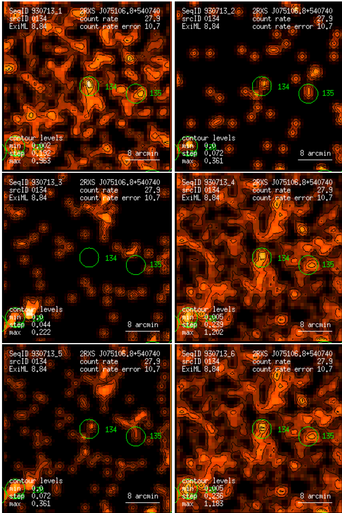
Figure 134: RASS 930713: detection 0134: band rate images, Gaussian filter: (1) PSPC channels 11 – 41, (2) 52 – 90, (3) 91 – 201, (4) 11 – 235, (5) 52 – 201, (6) 11 – 201. Broad band rates in counts/ks. Band rate contour levels in counts/ks/arcmin 2 .
