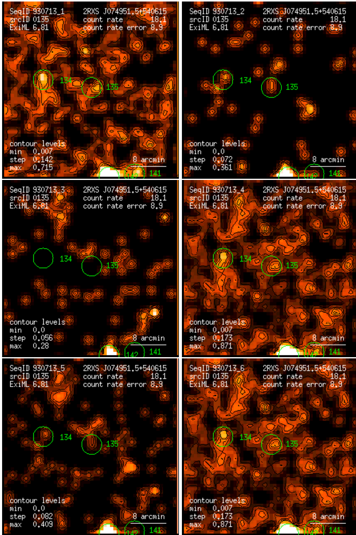
Figure 135: RASS 930713: detection 0135: band rate images, Gaussian filter: (1) PSPC channels 11 – 41, (2) 52 – 90, (3) 91 – 201, (4) 11 – 235, (5) 52 – 201, (6) 11 – 201. Broad band rates in counts/ks. Band rate contour levels in counts/ks/arcmin 2 .
