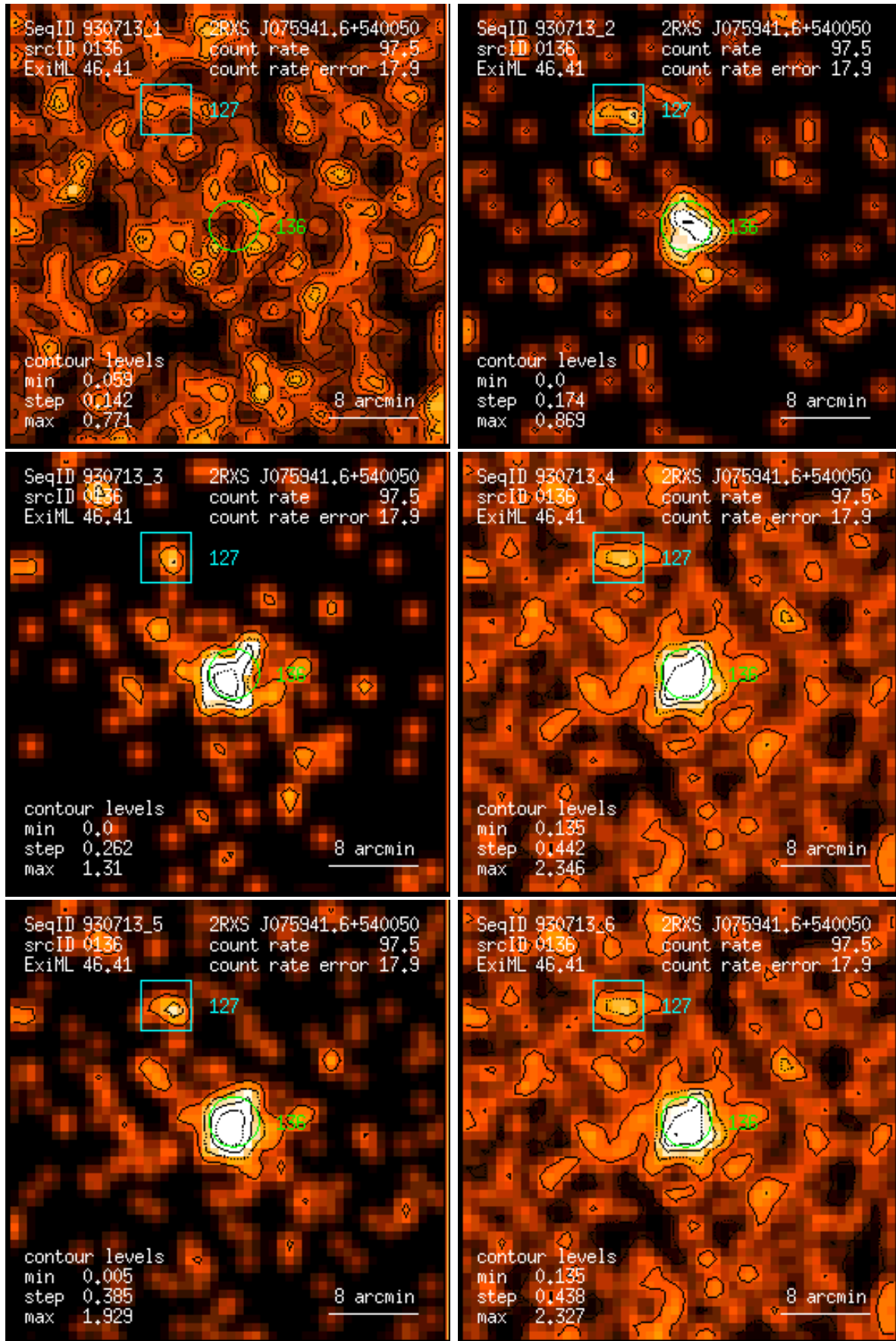
Figure 136: RASS 930713: detection 0136: band rate images, Gaussian filter: (1) PSPC channels 11 – 41, (2) 52 – 90, (3) 91 – 201, (4) 11 – 235, (5) 52 – 201, (6) 11 – 201. Broad band rates in counts/ks. Band rate contour levels in counts/ks/arcmin 2 .
