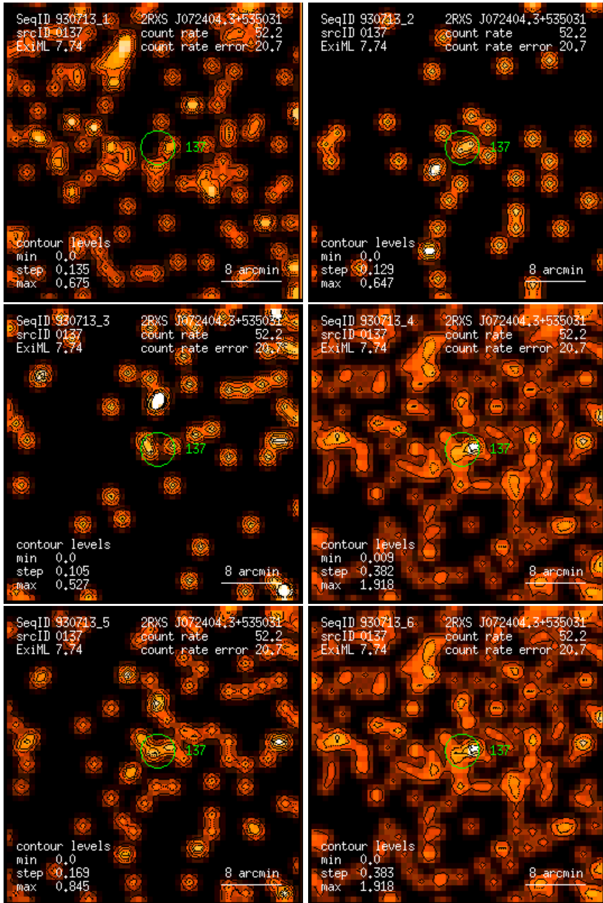
Figure 137: RASS 930713: detection 0137: band rate images, Gaussian filter: (1) PSPC channels 11 – 41, (2) 52 – 90, (3) 91 – 201, (4) 11 – 235, (5) 52 – 201, (6) 11 – 201. Broad band rates in counts/ks. Band rate contour levels in counts/ks/arcmin 2 .
