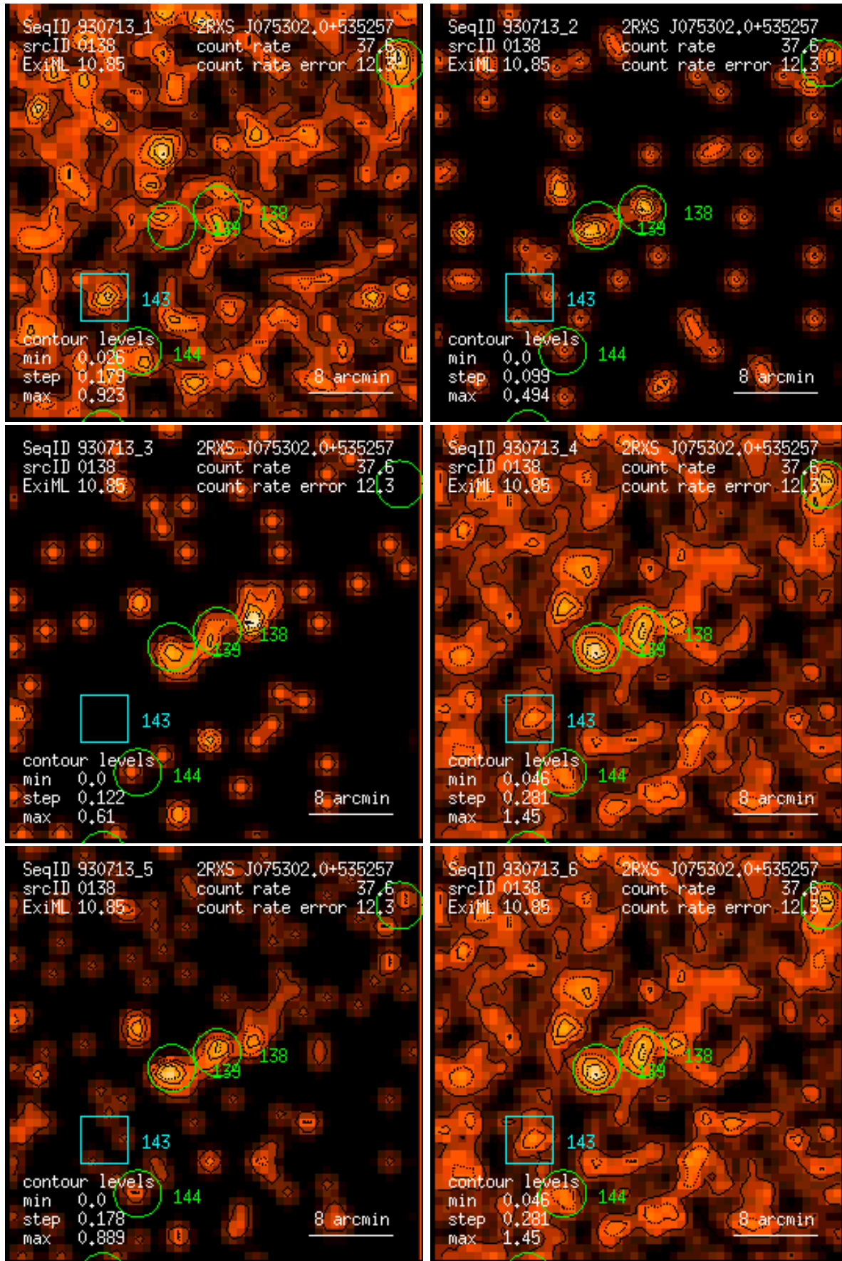
Figure 138: RASS 930713: detection 0138: band rate images, Gaussian filter: (1) PSPC channels 11 – 41, (2) 52 – 90, (3) 91 – 201, (4) 11 – 235, (5) 52 – 201, (6) 11 – 201. Broad band rates in counts/ks. Band rate contour levels in counts/ks/arcmin 2 .
