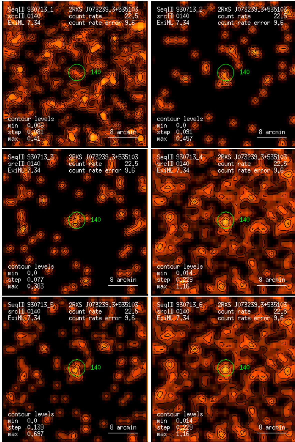
Figure 140: RASS 930713: detection 0140: band rate images, Gaussian filter: (1) PSPC channels 11 – 41, (2) 52 – 90, (3) 91 – 201, (4) 11 – 235, (5) 52 – 201, (6) 11 – 201. Broad band rates in counts/ks. Band rate contour levels in counts/ks/arcmin 2 .
