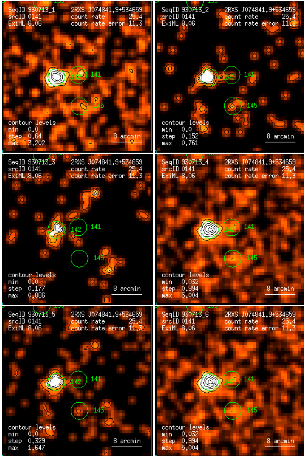
Figure 141: RASS 930713: detection 0141: band rate images, Gaussian filter: (1) PSPC channels 11 – 41, (2) 52 – 90, (3) 91 – 201, (4) 11 – 235, (5) 52 – 201, (6) 11 – 201. Broad band rates in counts/ks. Band rate contour levels in counts/ks/arcmin 2 .
