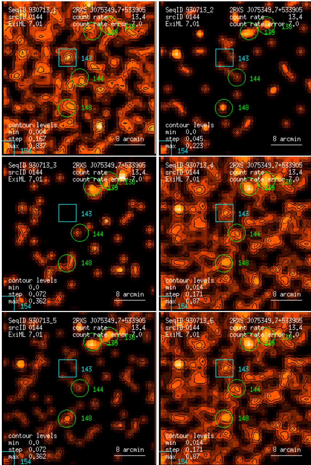
Figure 144: RASS 930713: detection 0144: band rate images, Gaussian filter: (1) PSPC channels 11 – 41, (2) 52 – 90, (3) 91 – 201, (4) 11 – 235, (5) 52 – 201, (6) 11 – 201. Broad band rates in counts/ks. Band rate contour levels in counts/ks/arcmin 2 .
