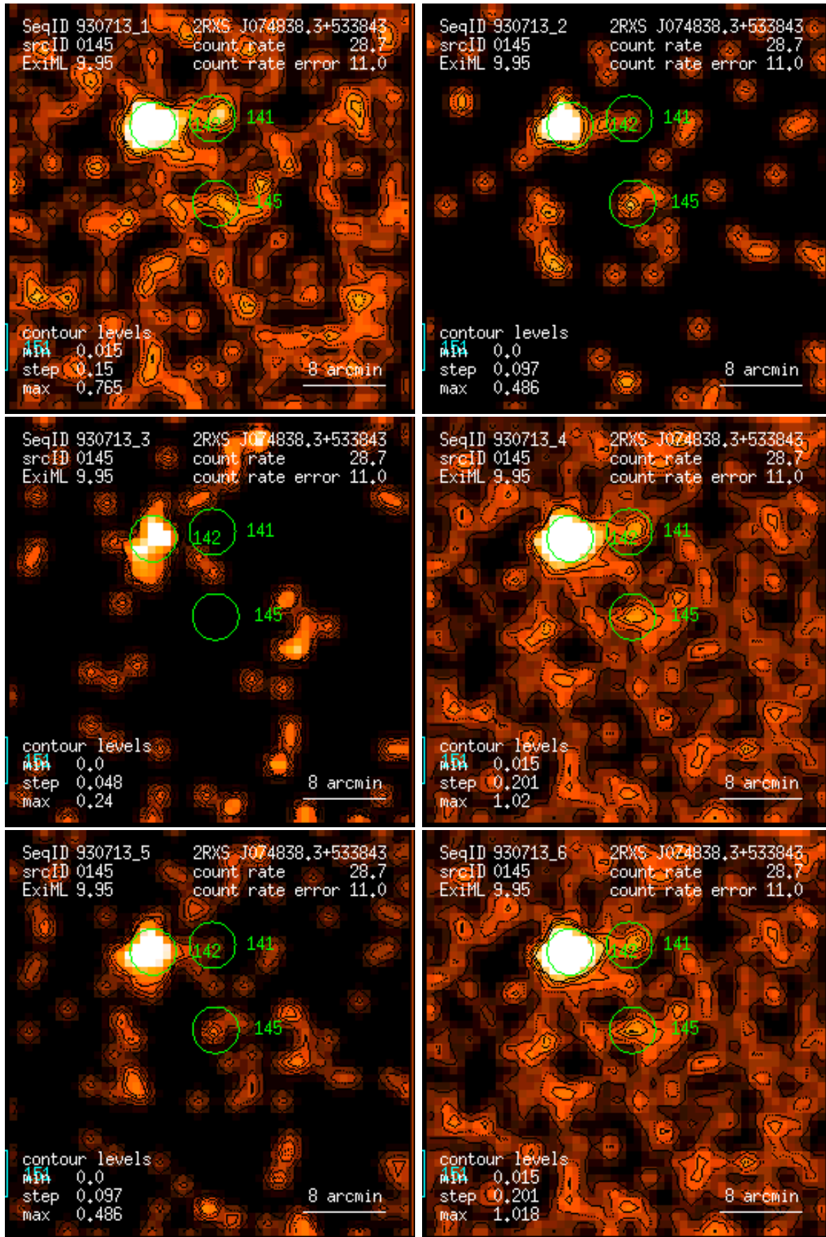
Figure 145: RASS 930713: detection 0145: band rate images, Gaussian filter: (1) PSPC channels 11 – 41, (2) 52 – 90, (3) 91 – 201, (4) 11 – 235, (5) 52 – 201, (6) 11 – 201. Broad band rates in counts/ks. Band rate contour levels in counts/ks/arcmin 2 .
