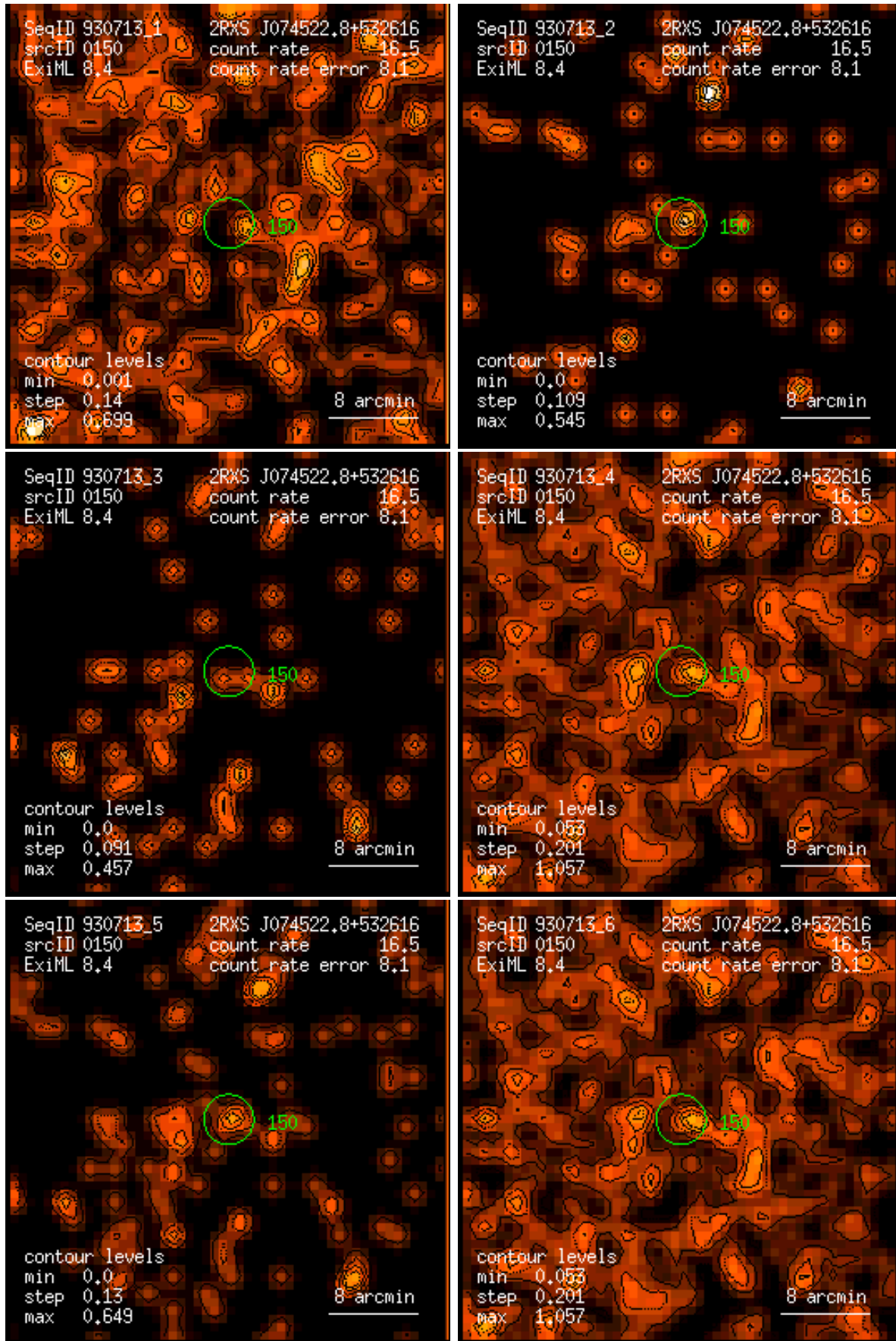
Figure 150: RASS 930713: detection 0150: band rate images, Gaussian filter: (1) PSPC channels 11 – 41, (2) 52 – 90, (3) 91 – 201, (4) 11 – 235, (5) 52 – 201, (6) 11 – 201. Broad band rates in counts/ks. Band rate contour levels in counts/ks/arcmin 2 .
