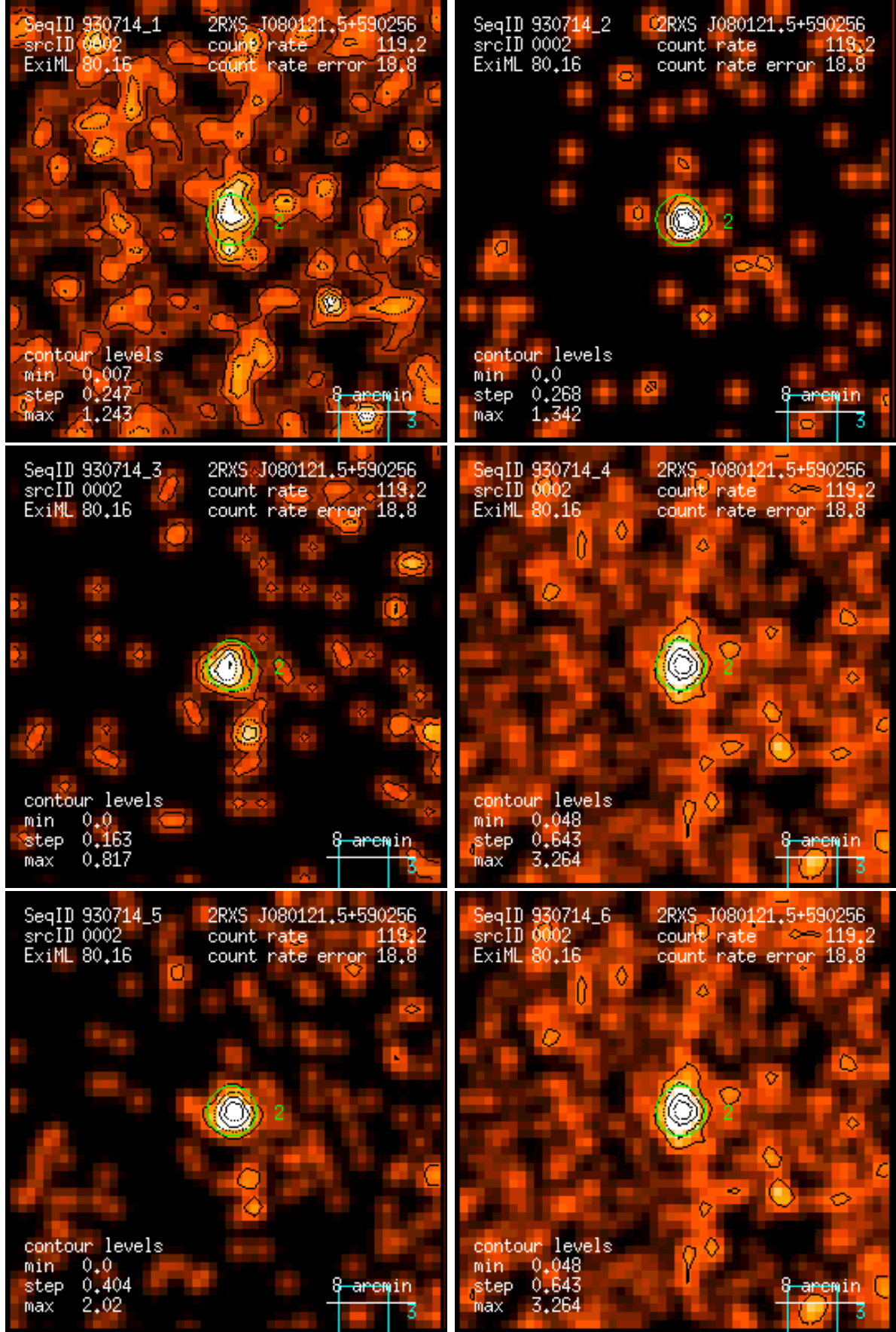
Figure 2: RASS 930714: detection 0002: band rate images, Gaussian filter: (1) PSPC channels 11 – 41, (2) 52 – 90, (3) 91 – 201, (4) 11 – 235, (5) 52 – 201, (6) 11 – 201. Broad band rates in counts/ks. Band rate contour levels in counts/ks/arcmin 2 .
