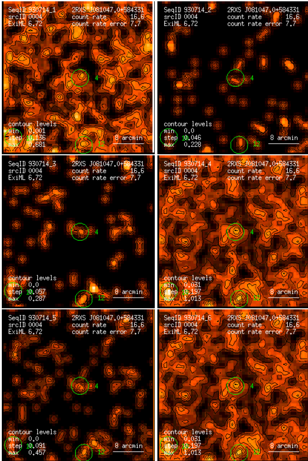
Figure 4: RASS 930714: detection 0004: band rate images, Gaussian filter: (1) PSPC channels 11 – 41, (2) 52 – 90, (3) 91 – 201, (4) 11 – 235, (5) 52 – 201, (6) 11 – 201. Broad band rates in counts/ks. Band rate contour levels in counts/ks/arcmin 2 .
