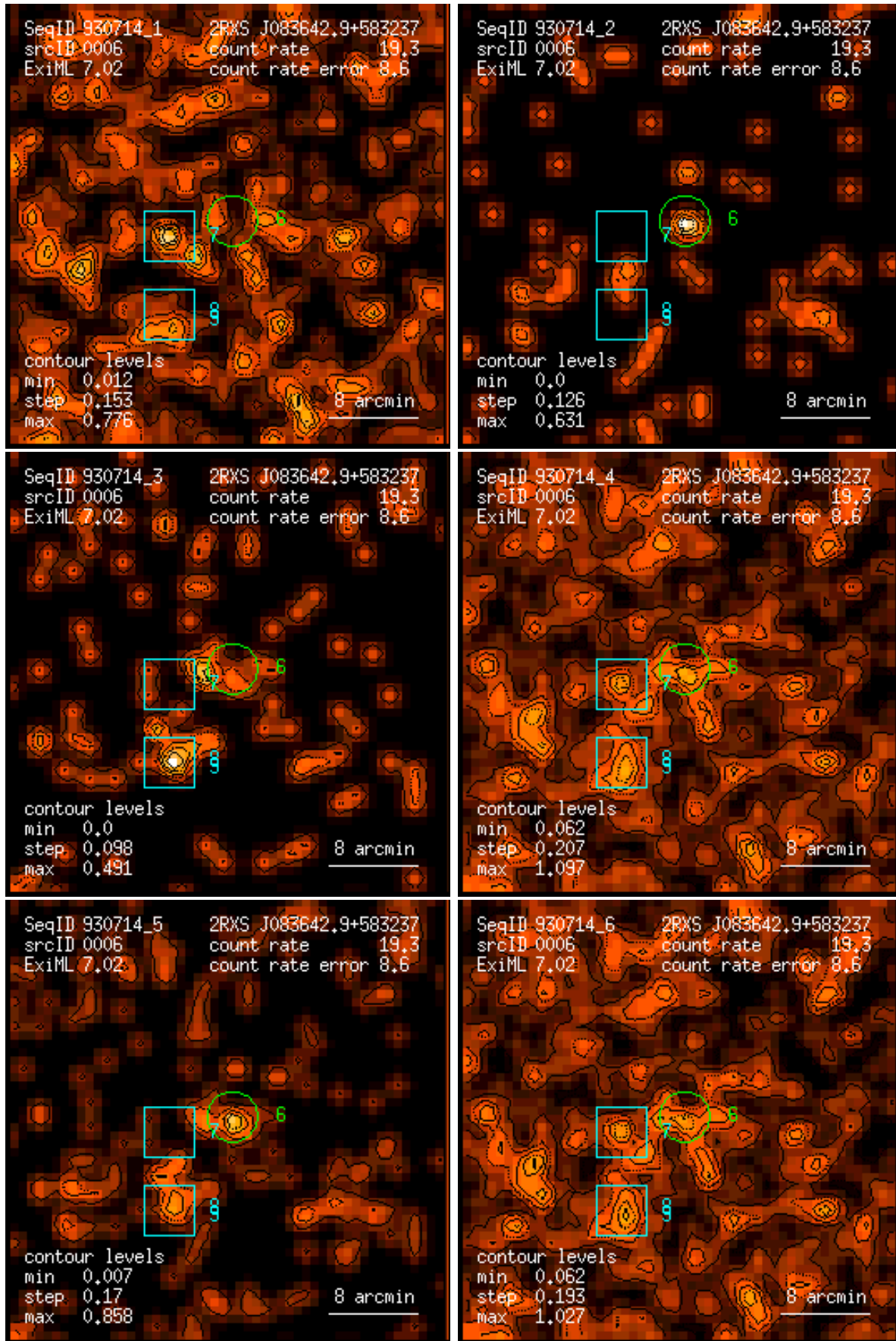
Figure 6: RASS 930714: detection 0006: band rate images, Gaussian filter: (1) PSPC channels 11 – 41, (2) 52 – 90, (3) 91 – 201, (4) 11 – 235, (5) 52 – 201, (6) 11 – 201. Broad band rates in counts/ks. Band rate contour levels in counts/ks/arcmin 2 .
