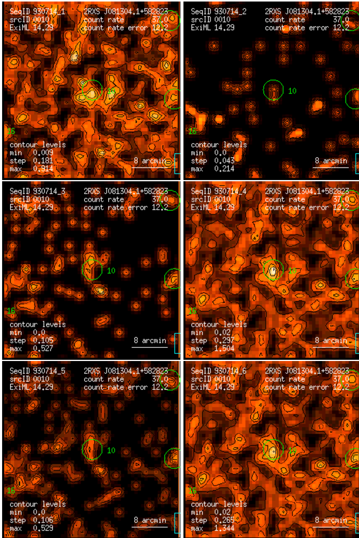
Figure 10: RASS 930714: detection 0010: band rate images, Gaussian filter: (1) PSPC channels 11 – 41, (2) 52 – 90, (3) 91 – 201, (4) 11 – 235, (5) 52 – 201, (6) 11 – 201. Broad band rates in counts/ks. Band rate contour levels in counts/ks/arcmin 2 .
