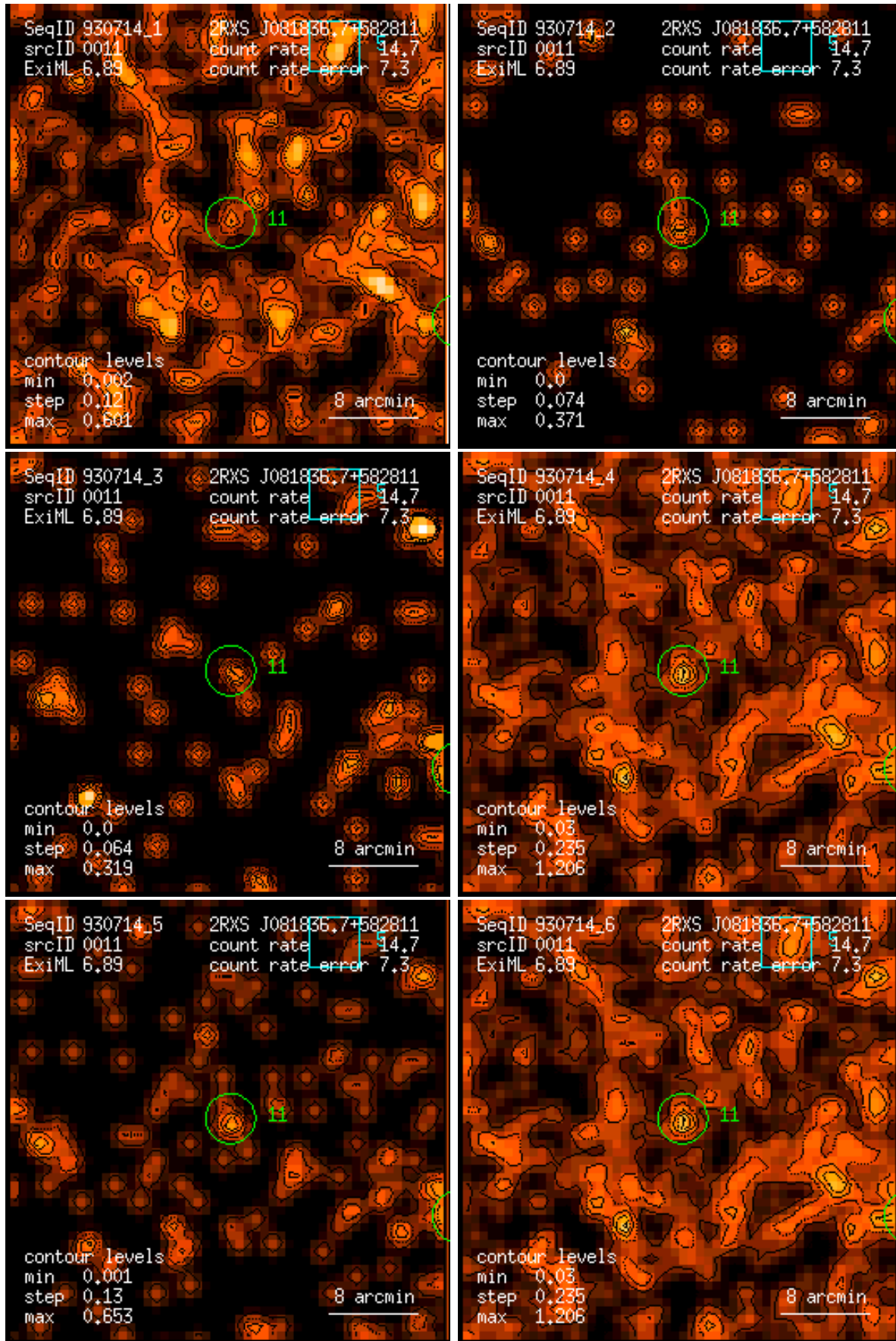
Figure 11: RASS 930714: detection 0011: band rate images, Gaussian filter: (1) PSPC channels 11 – 41, (2) 52 – 90, (3) 91 – 201, (4) 11 – 235, (5) 52 – 201, (6) 11 – 201. Broad band rates in counts/ks. Band rate contour levels in counts/ks/arcmin 2 .
