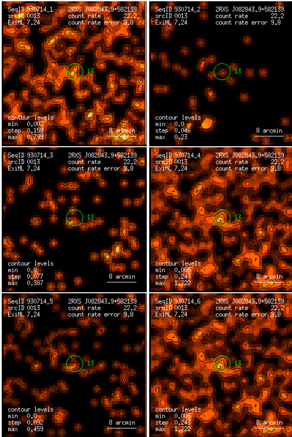
Figure 13: RASS 930714: detection 0013: band rate images, Gaussian filter: (1) PSPC channels 11 – 41, (2) 52 – 90, (3) 91 – 201, (4) 11 – 235, (5) 52 – 201, (6) 11 – 201. Broad band rates in counts/ks. Band rate contour levels in counts/ks/arcmin 2 .
