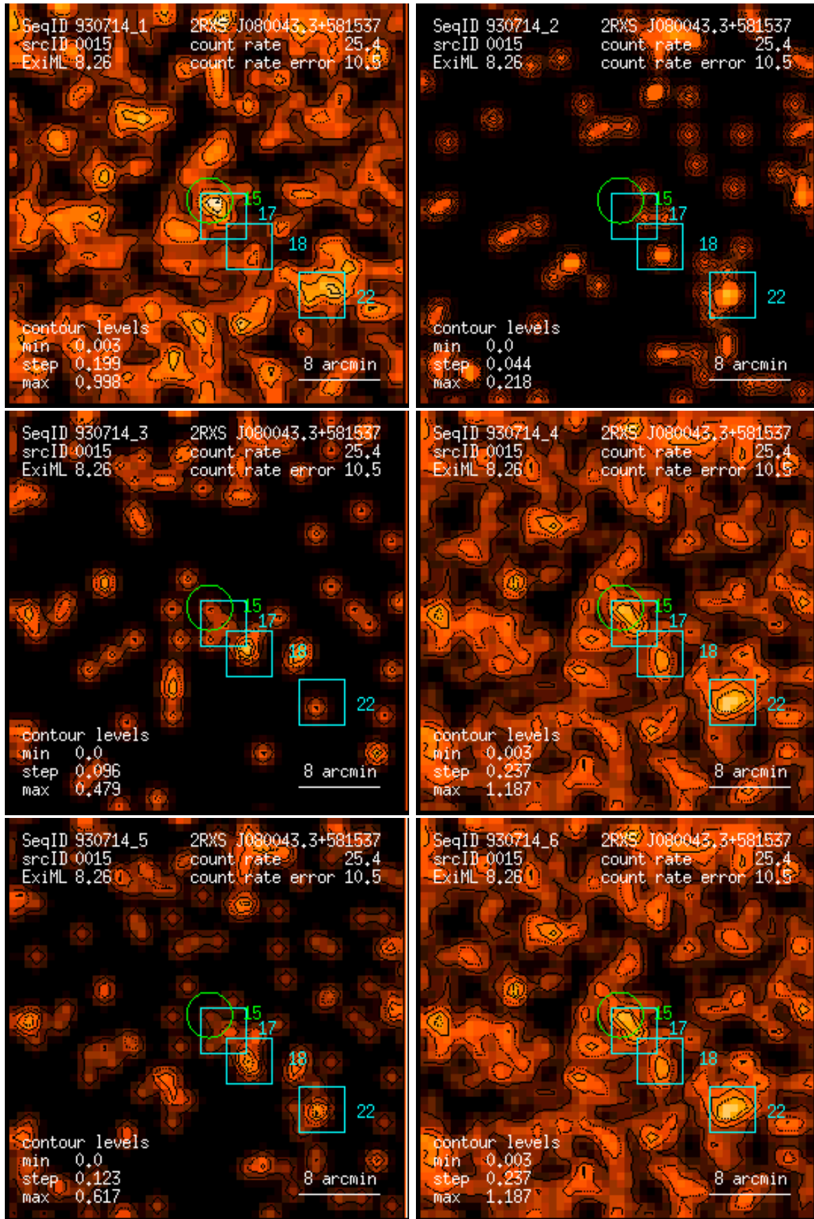
Figure 15: RASS 930714: detection 0015: band rate images, Gaussian filter: (1) PSPC channels 11 – 41, (2) 52 – 90, (3) 91 – 201, (4) 11 – 235, (5) 52 – 201, (6) 11 – 201. Broad band rates in counts/ks. Band rate contour levels in counts/ks/arcmin 2 .
