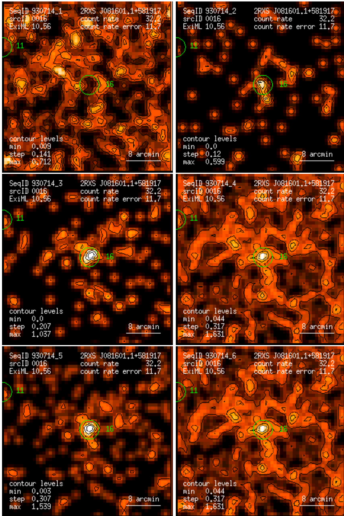
Figure 16: RASS 930714: detection 0016: band rate images, Gaussian filter: (1) PSPC channels 11 – 41, (2) 52 – 90, (3) 91 – 201, (4) 11 – 235, (5) 52 – 201, (6) 11 – 201. Broad band rates in counts/ks. Band rate contour levels in counts/ks/arcmin 2 .
