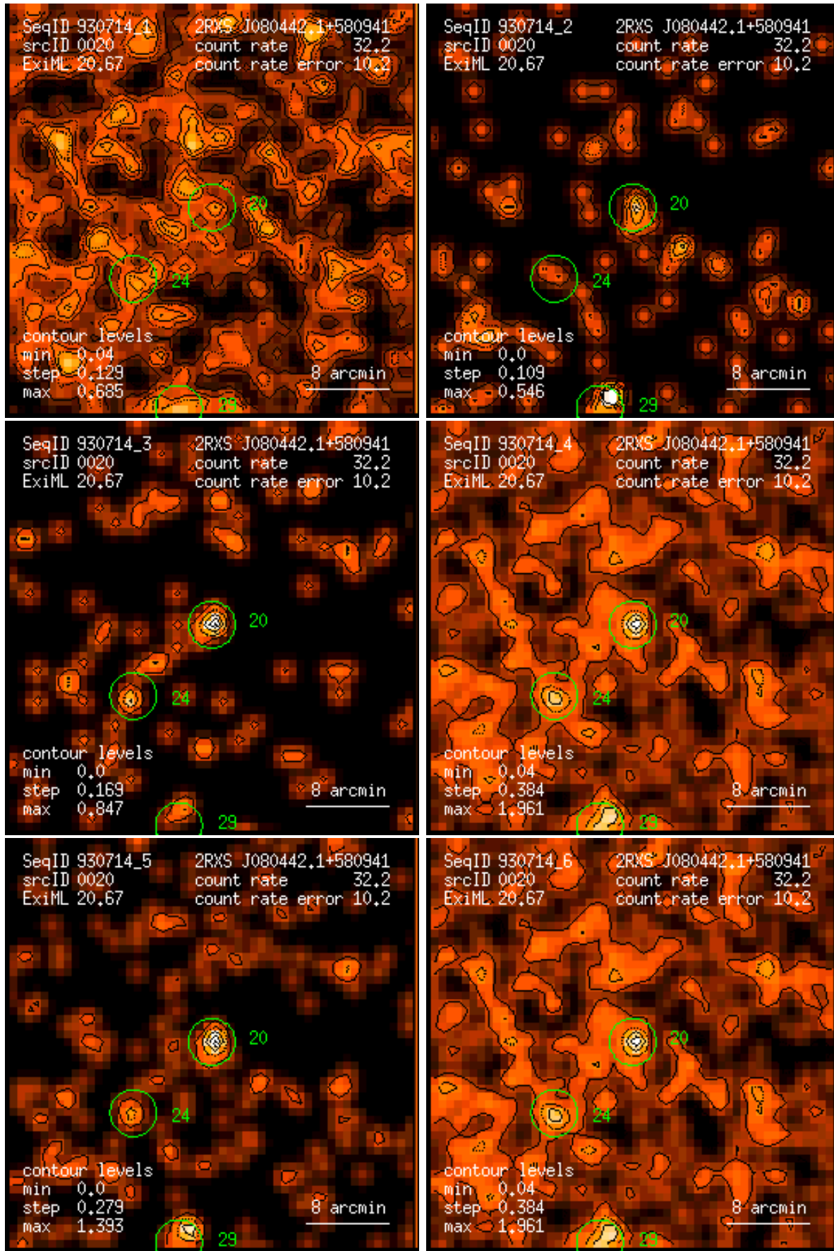
Figure 20: RASS 930714: detection 0020: band rate images, Gaussian filter: (1) PSPC channels 11 – 41, (2) 52 – 90, (3) 91 – 201, (4) 11 – 235, (5) 52 – 201, (6) 11 – 201. Broad band rates in counts/ks. Band rate contour levels in counts/ks/arcmin 2 .
