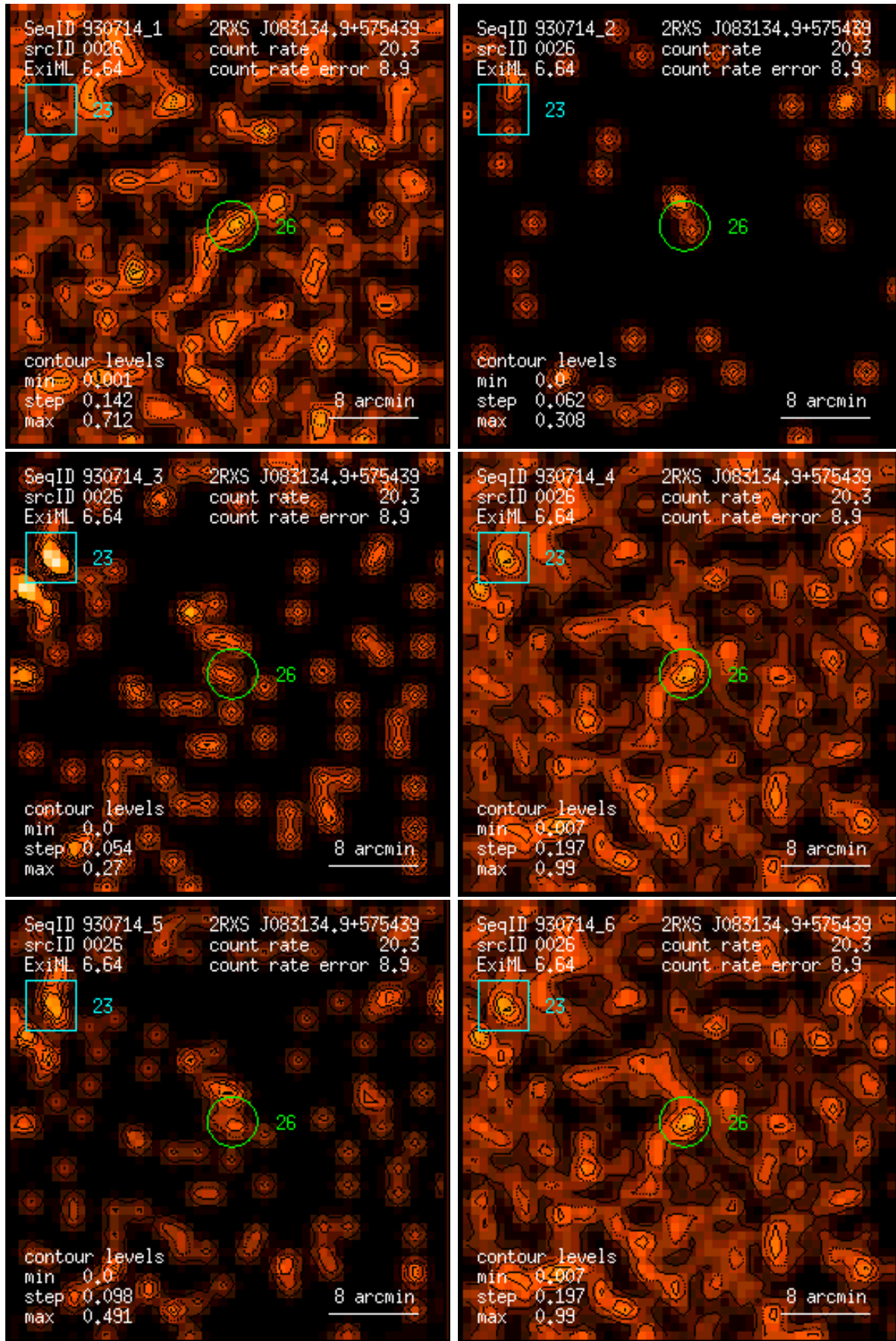
Figure 26: RASS 930714: detection 0026: band rate images, Gaussian filter: (1) PSPC channels 11 – 41, (2) 52 – 90, (3) 91 – 201, (4) 11 – 235, (5) 52 – 201, (6) 11 – 201. Broad band rates in counts/ks. Band rate contour levels in counts/ks/arcmin 2 .
