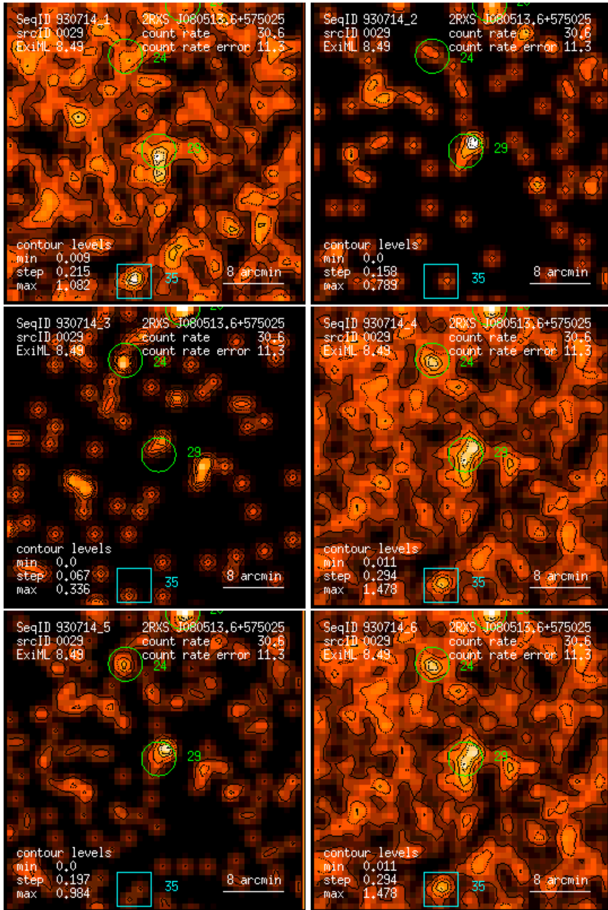
Figure 29: RASS 930714: detection 0029: band rate images, Gaussian filter: (1) PSPC channels 11 – 41, (2) 52 – 90, (3) 91 – 201, (4) 11 – 235, (5) 52 – 201, (6) 11 – 201. Broad band rates in counts/ks. Band rate contour levels in counts/ks/arcmin 2 .
