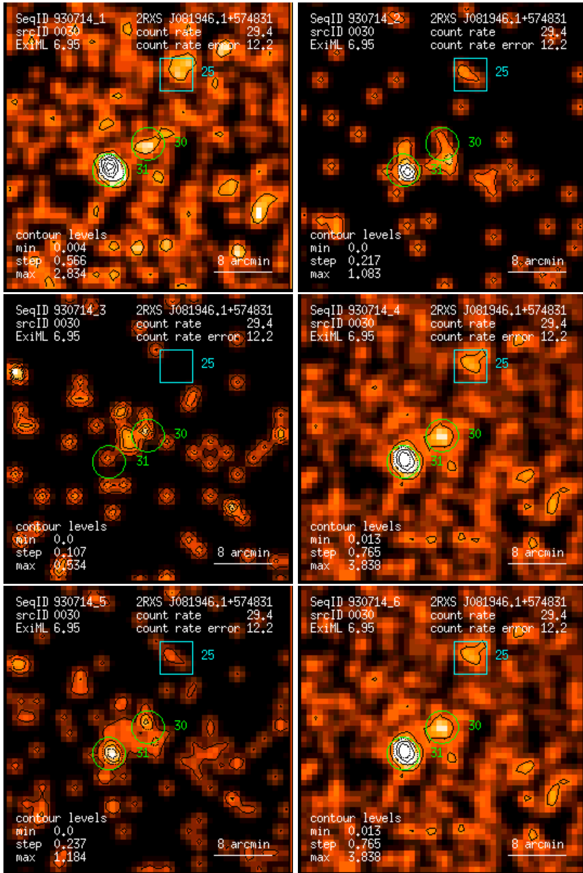
Figure 30: RASS 930714: detection 0030: band rate images, Gaussian filter: (1) PSPC channels 11 – 41, (2) 52 – 90, (3) 91 – 201, (4) 11 – 235, (5) 52 – 201, (6) 11 – 201. Broad band rates in counts/ks. Band rate contour levels in counts/ks/arcmin 2 .
