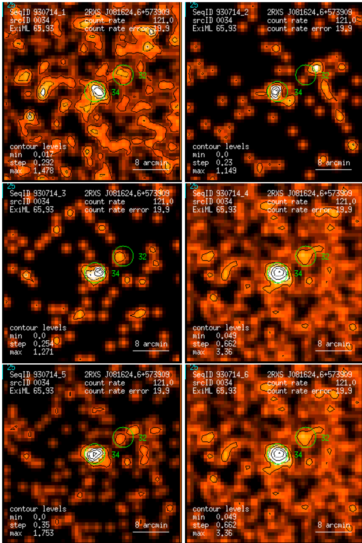
Figure 34: RASS 930714: detection 0034: band rate images, Gaussian filter: (1) PSPC channels 11 – 41, (2) 52 – 90, (3) 91 – 201, (4) 11 – 235, (5) 52 – 201, (6) 11 – 201. Broad band rates in counts/ks. Band rate contour levels in counts/ks/arcmin 2 .
