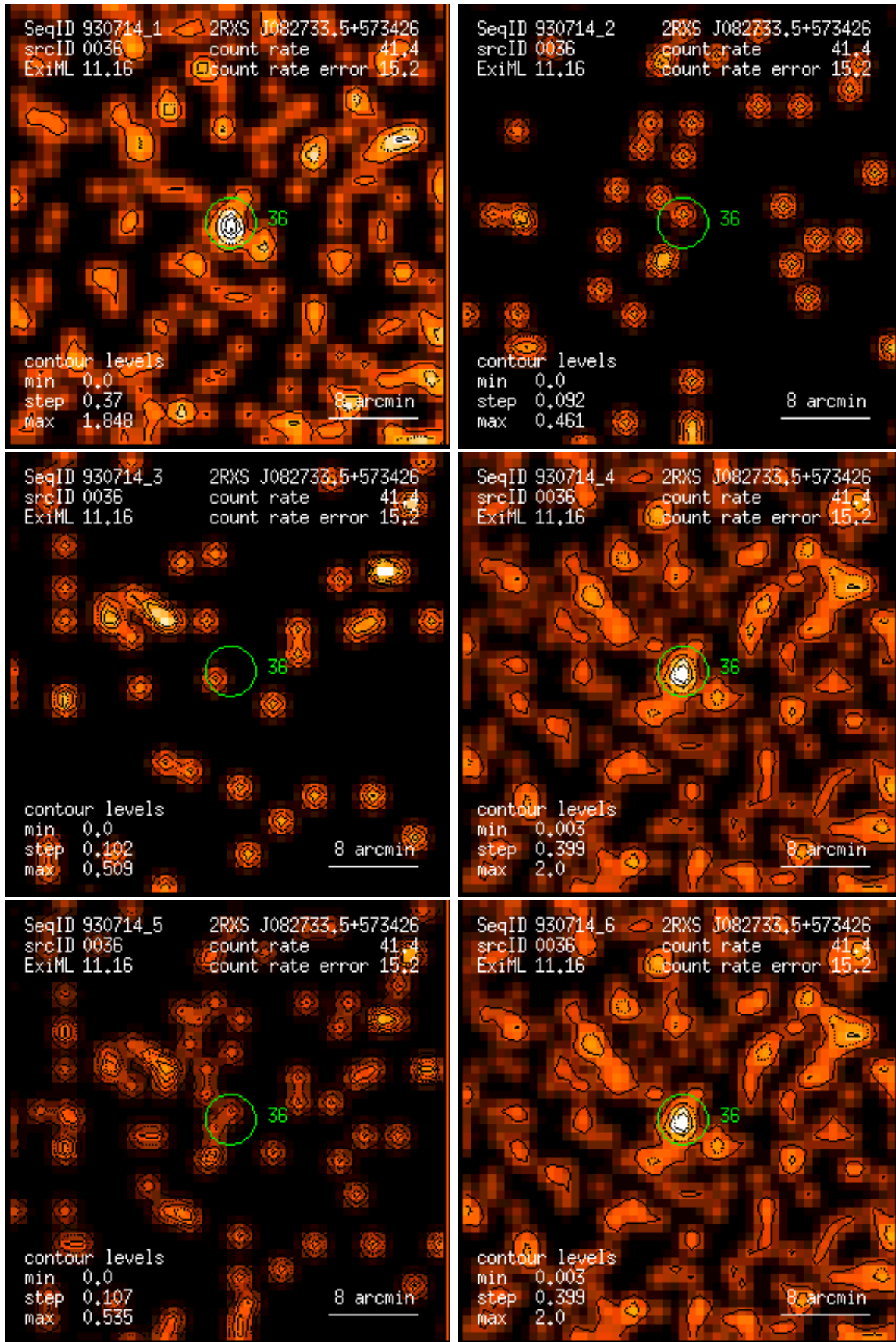
Figure 36: RASS 930714: detection 0036: band rate images, Gaussian filter: (1) PSPC channels 11 – 41, (2) 52 – 90, (3) 91 – 201, (4) 11 – 235, (5) 52 – 201, (6) 11 – 201. Broad band rates in counts/ks. Band rate contour levels in counts/ks/arcmin 2 .
