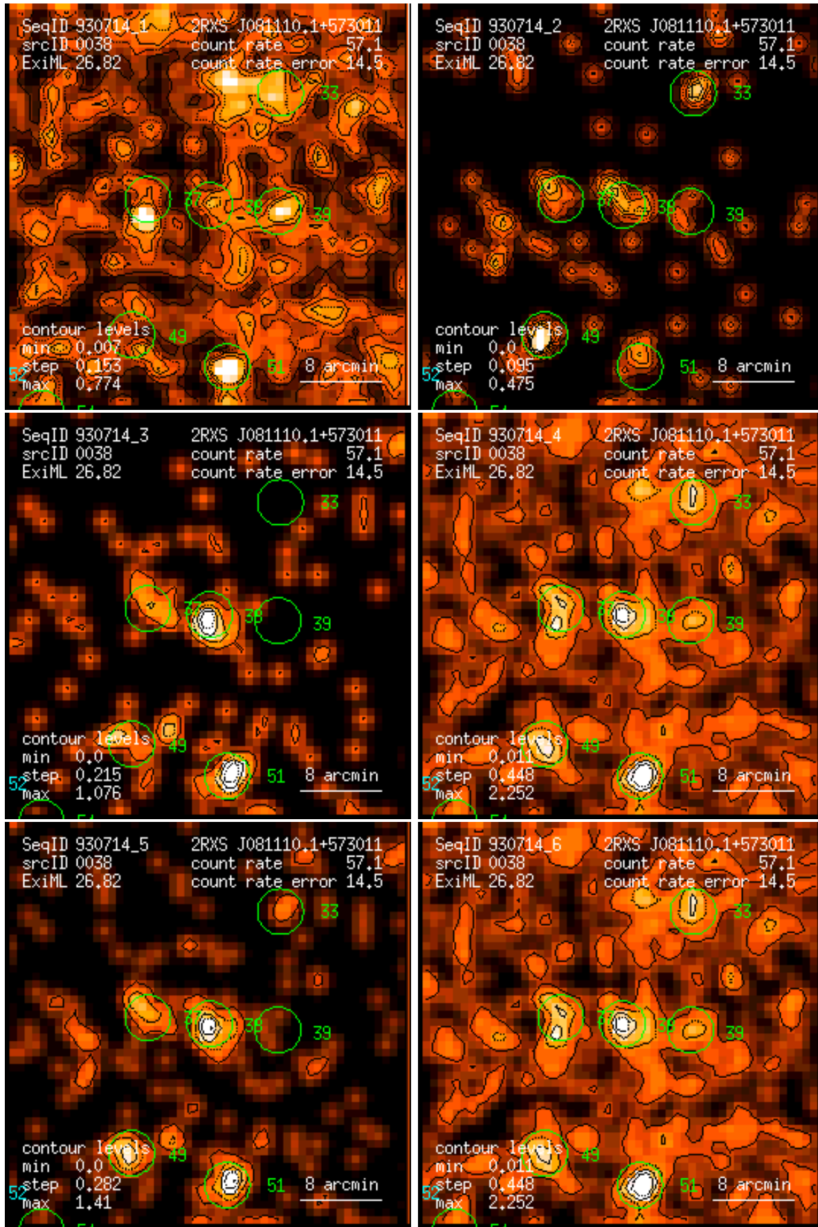
Figure 38: RASS 930714: detection 0038: band rate images, Gaussian filter: (1) PSPC channels 11 – 41, (2) 52 – 90, (3) 91 – 201, (4) 11 – 235, (5) 52 – 201, (6) 11 – 201. Broad band rates in counts/ks. Band rate contour levels in counts/ks/arcmin 2 .
