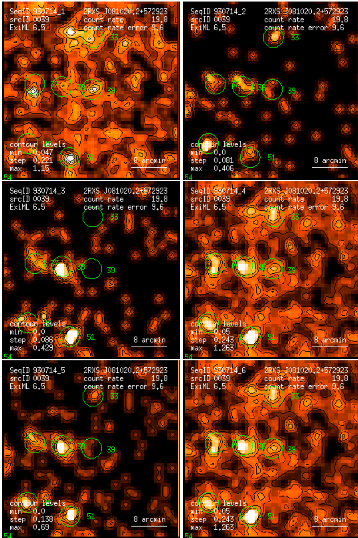
Figure 39: RASS 930714: detection 0039: band rate images, Gaussian filter: (1) PSPC channels 11 – 41, (2) 52 – 90, (3) 91 – 201, (4) 11 – 235, (5) 52 – 201, (6) 11 – 201. Broad band rates in counts/ks. Band rate contour levels in counts/ks/arcmin 2 .
