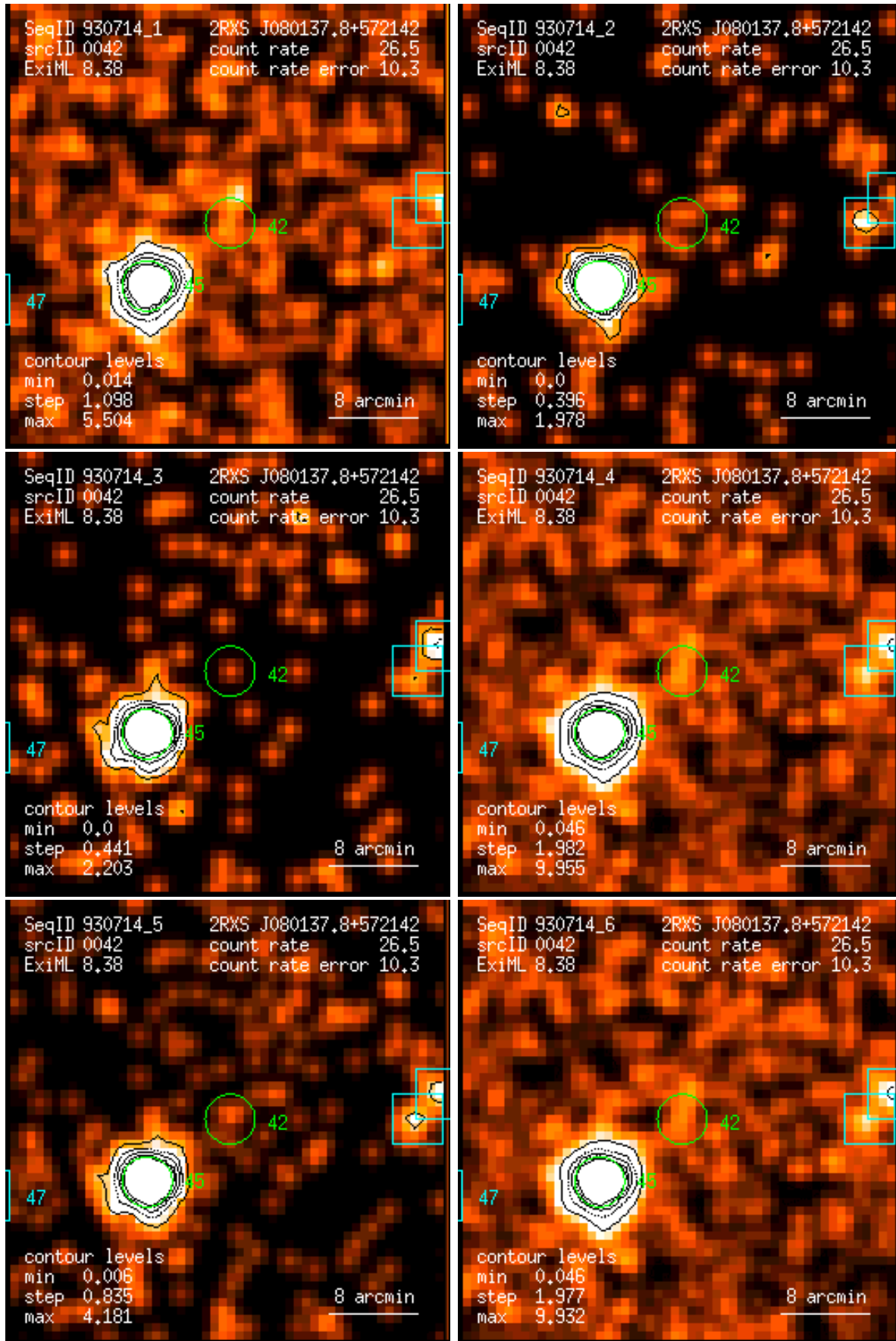
Figure 42: RASS 930714: detection 0042: band rate images, Gaussian filter: (1) PSPC channels 11 – 41, (2) 52 – 90, (3) 91 – 201, (4) 11 – 235, (5) 52 – 201, (6) 11 – 201. Broad band rates in counts/ks. Band rate contour levels in counts/ks/arcmin 2 .
