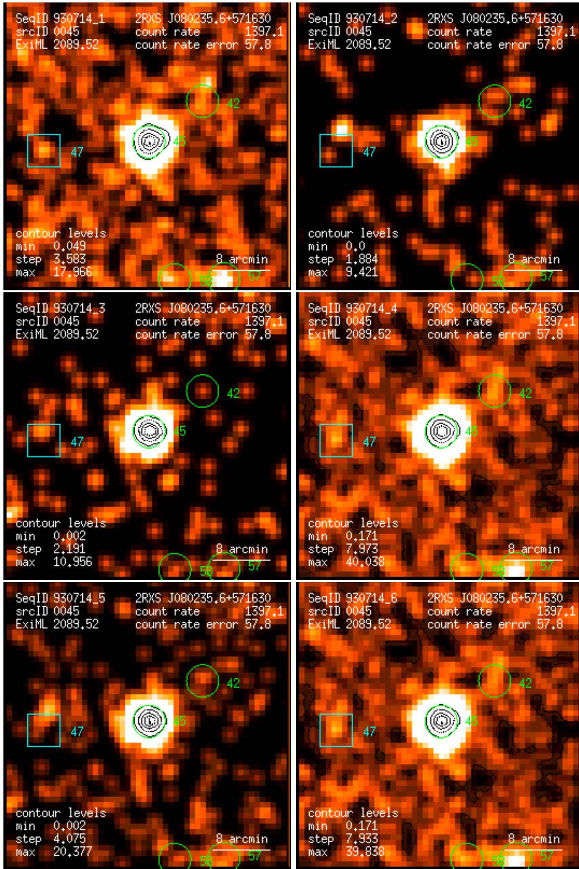
Figure 45: RASS 930714: detection 0045: band rate images, Gaussian filter: (1) PSPC channels 11 – 41, (2) 52 – 90, (3) 91 – 201, (4) 11 – 235, (5) 52 – 201, (6) 11 – 201. Broad band rates in counts/ks. Band rate contour levels in counts/ks/arcmin 2 .
