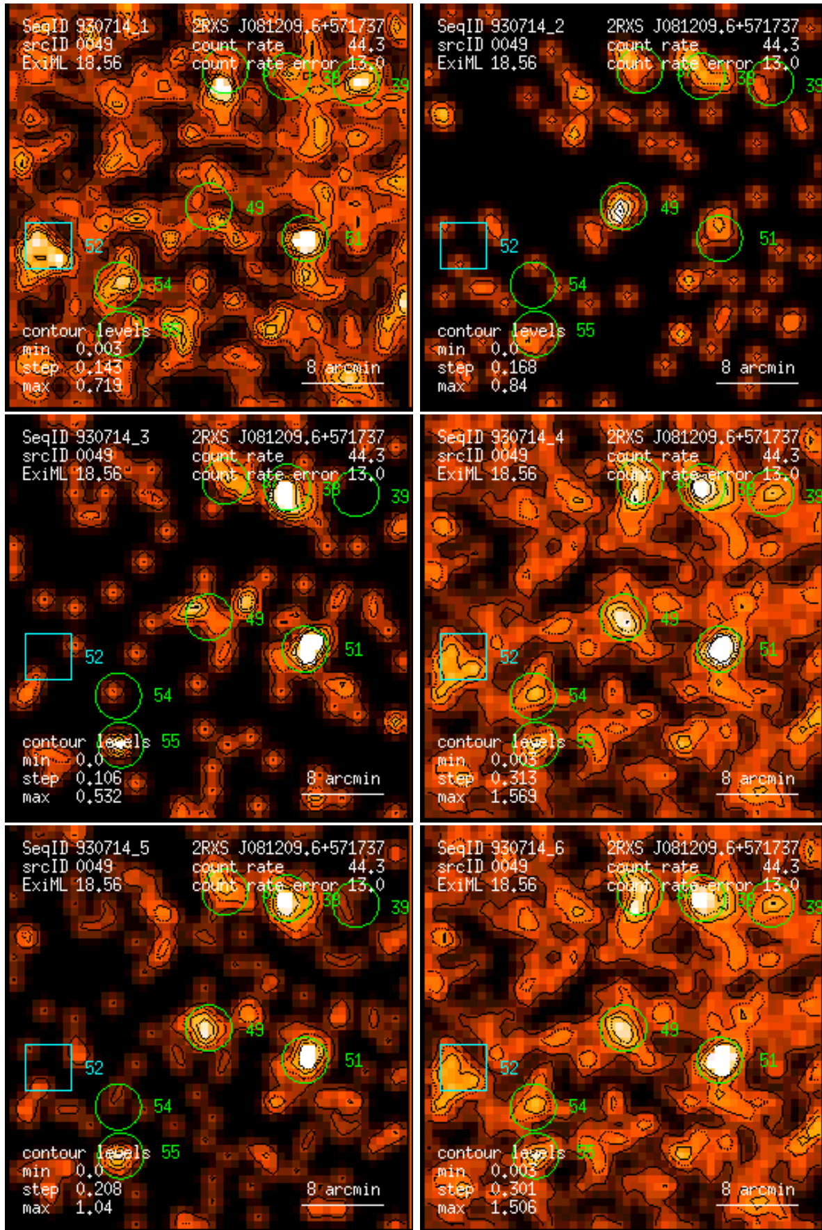
Figure 49: RASS 930714: detection 0049: band rate images, Gaussian filter: (1) PSPC channels 11 – 41, (2) 52 – 90, (3) 91 – 201, (4) 11 – 235, (5) 52 – 201, (6) 11 – 201. Broad band rates in counts/ks. Band rate contour levels in counts/ks/arcmin 2 .
