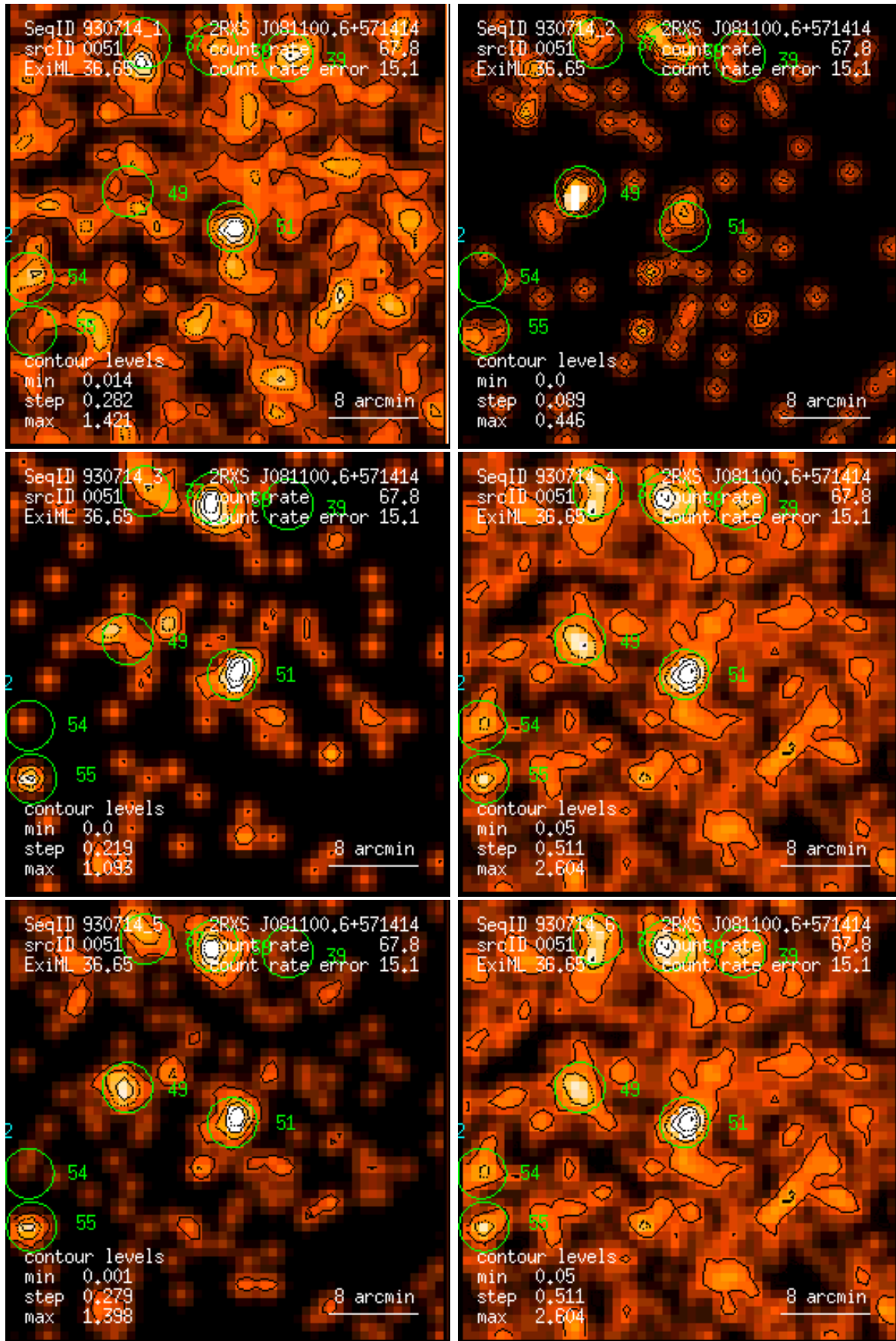
Figure 51: RASS 930714: detection 0051: band rate images, Gaussian filter: (1) PSPC channels 11 – 41, (2) 52 – 90, (3) 91 – 201, (4) 11 – 235, (5) 52 – 201, (6) 11 – 201. Broad band rates in counts/ks. Band rate contour levels in counts/ks/arcmin 2 .
