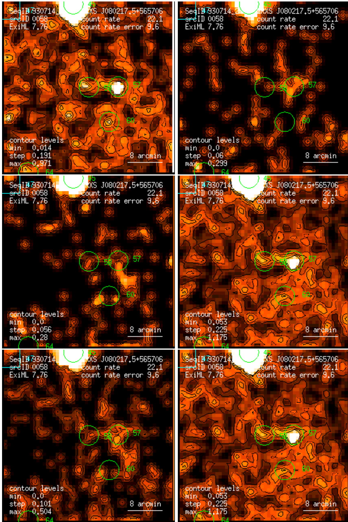
Figure 58: RASS 930714: detection 0058: band rate images, Gaussian filter: (1) PSPC channels 11 – 41, (2) 52 – 90, (3) 91 – 201, (4) 11 – 235, (5) 52 – 201, (6) 11 – 201. Broad band rates in counts/ks. Band rate contour levels in counts/ks/arcmin 2 .
