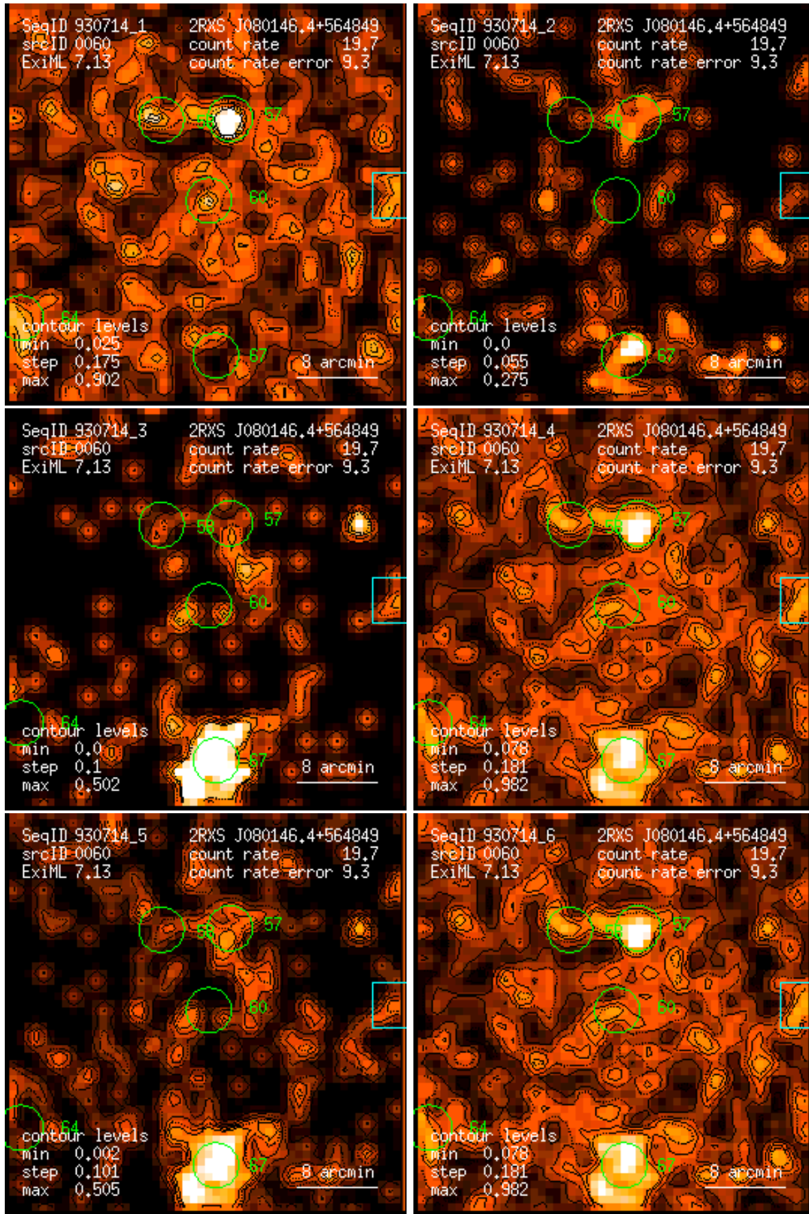
Figure 60: RASS 930714: detection 0060: band rate images, Gaussian filter: (1) PSPC channels 11 – 41, (2) 52 – 90, (3) 91 – 201, (4) 11 – 235, (5) 52 – 201, (6) 11 – 201. Broad band rates in counts/ks. Band rate contour levels in counts/ks/arcmin 2 .
