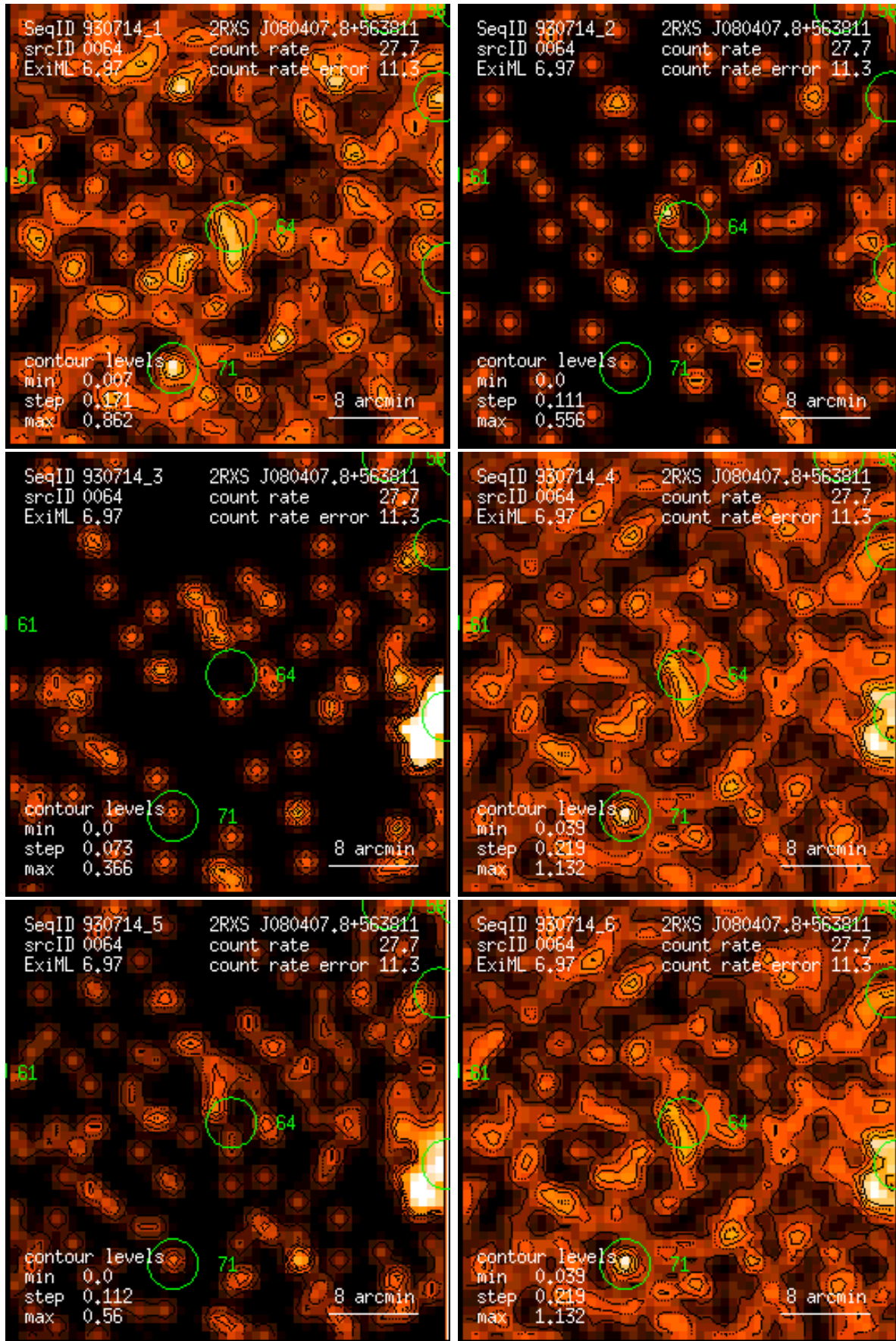
Figure 64: RASS 930714: detection 0064: band rate images, Gaussian filter: (1) PSPC channels 11 – 41, (2) 52 – 90, (3) 91 – 201, (4) 11 – 235, (5) 52 – 201, (6) 11 – 201. Broad band rates in counts/ks. Band rate contour levels in counts/ks/arcmin 2 .
