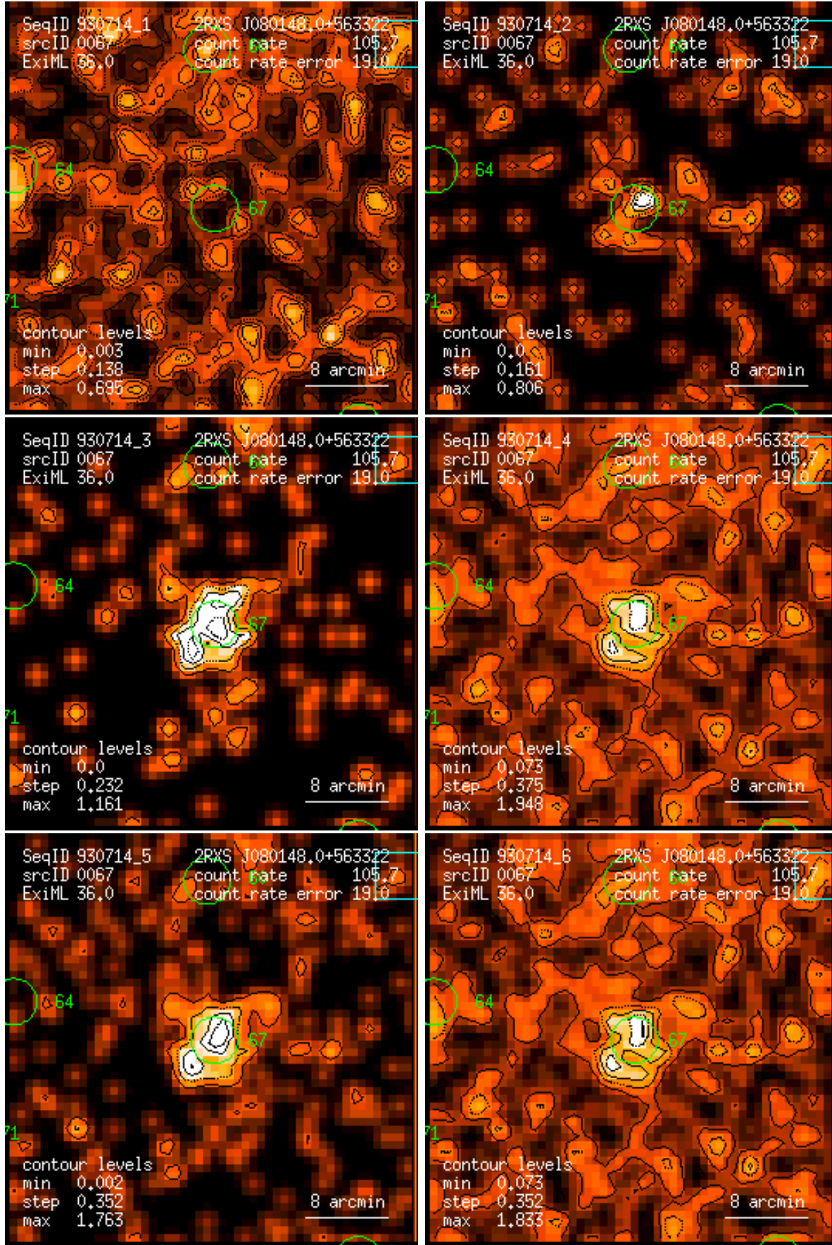
Figure 67: RASS 930714: detection 0067: band rate images, Gaussian filter: (1) PSPC channels 11 – 41, (2) 52 – 90, (3) 91 – 201, (4) 11 – 235, (5) 52 – 201, (6) 11 – 201. Broad band rates in counts/ks. Band rate contour levels in counts/ks/arcmin 2 .
