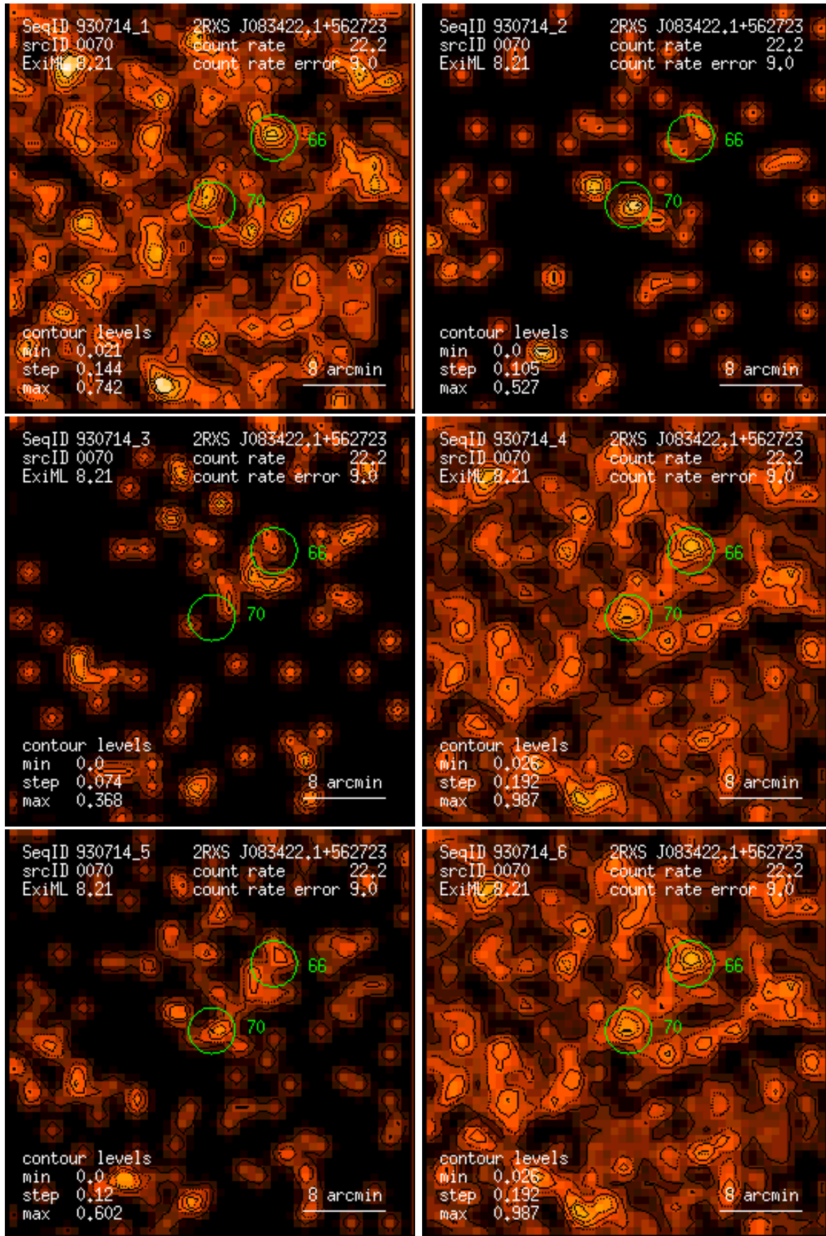
Figure 70: RASS 930714: detection 0070: band rate images, Gaussian filter: (1) PSPC channels 11 – 41, (2) 52 – 90, (3) 91 – 201, (4) 11 – 235, (5) 52 – 201, (6) 11 – 201. Broad band rates in counts/ks. Band rate contour levels in counts/ks/arcmin 2 .
