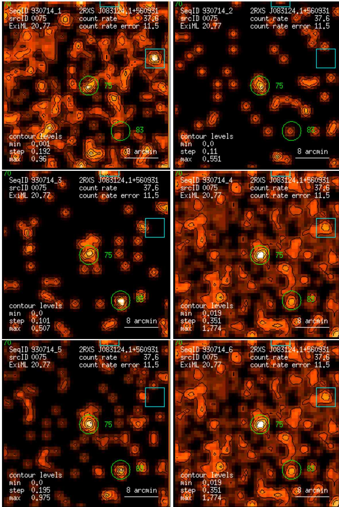
Figure 75: RASS 930714: detection 0075: band rate images, Gaussian filter: (1) PSPC channels 11 – 41, (2) 52 – 90, (3) 91 – 201, (4) 11 – 235, (5) 52 – 201, (6) 11 – 201. Broad band rates in counts/ks. Band rate contour levels in counts/ks/arcmin 2 .
