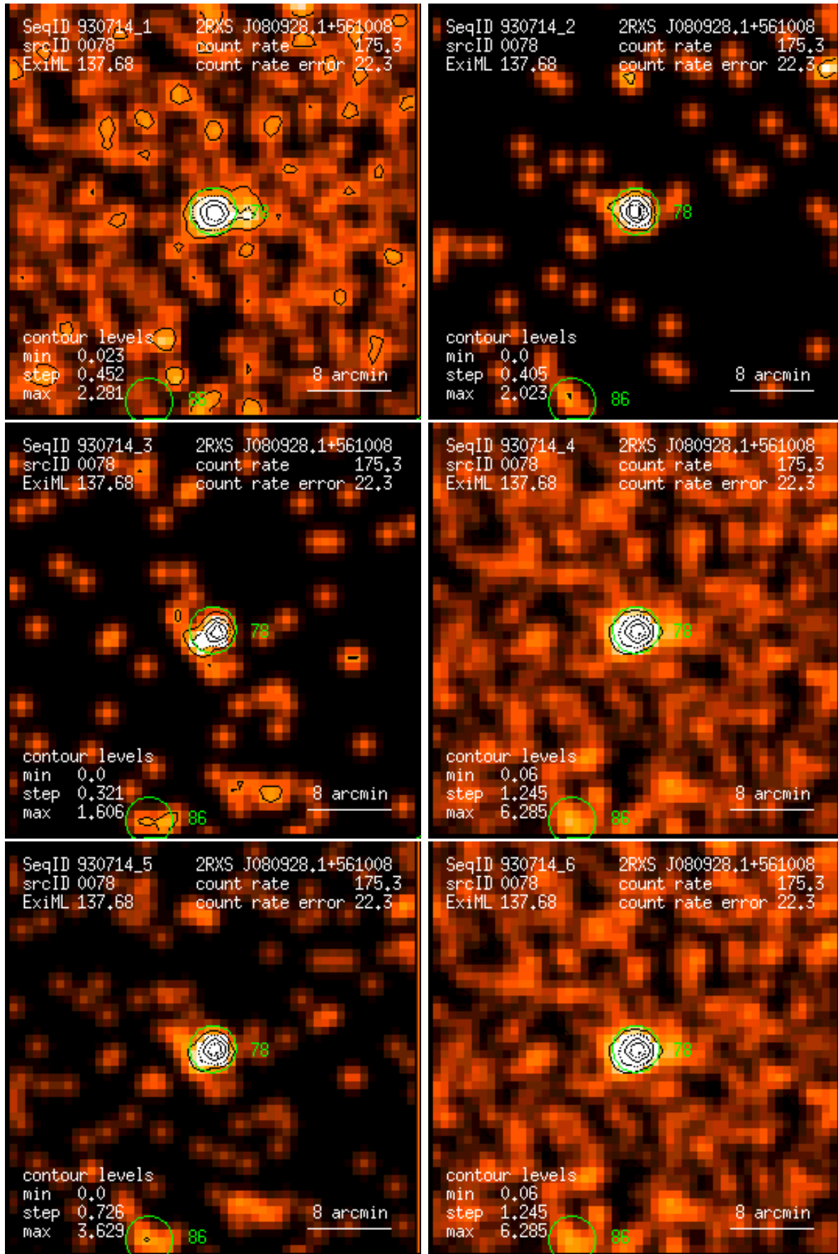
Figure 78: RASS 930714: detection 0078: band rate images, Gaussian filter: (1) PSPC channels 11 – 41, (2) 52 – 90, (3) 91 – 201, (4) 11 – 235, (5) 52 – 201, (6) 11 – 201. Broad band rates in counts/ks. Band rate contour levels in counts/ks/arcmin 2 .
