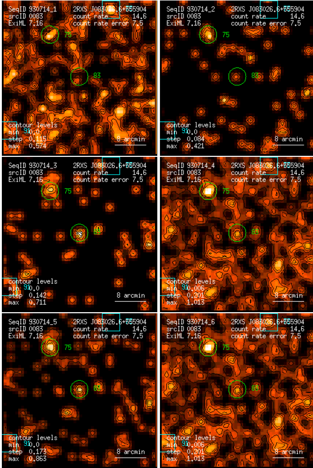
Figure 83: RASS 930714: detection 0083: band rate images, Gaussian filter: (1) PSPC channels 11 – 41, (2) 52 – 90, (3) 91 – 201, (4) 11 – 235, (5) 52 – 201, (6) 11 – 201. Broad band rates in counts/ks. Band rate contour levels in counts/ks/arcmin 2 .
