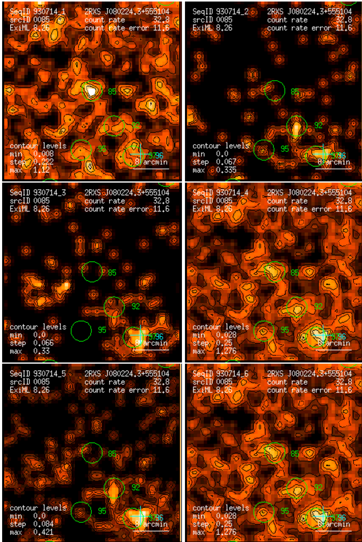
Figure 85: RASS 930714: detection 0085: band rate images, Gaussian filter: (1) PSPC channels 11 – 41, (2) 52 – 90, (3) 91 – 201, (4) 11 – 235, (5) 52 – 201, (6) 11 – 201. Broad band rates in counts/ks. Band rate contour levels in counts/ks/arcmin 2 .
