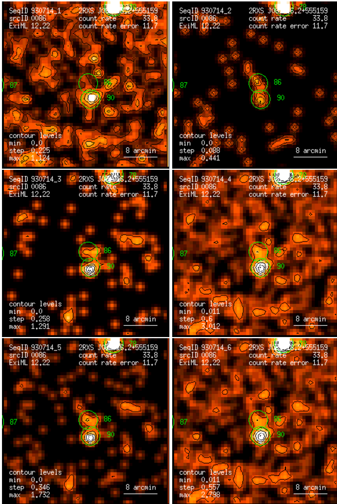
Figure 86: RASS 930714: detection 0086: band rate images, Gaussian filter: (1) PSPC channels 11 – 41, (2) 52 – 90, (3) 91 – 201, (4) 11 – 235, (5) 52 – 201, (6) 11 – 201. Broad band rates in counts/ks. Band rate contour levels in counts/ks/arcmin 2 .
