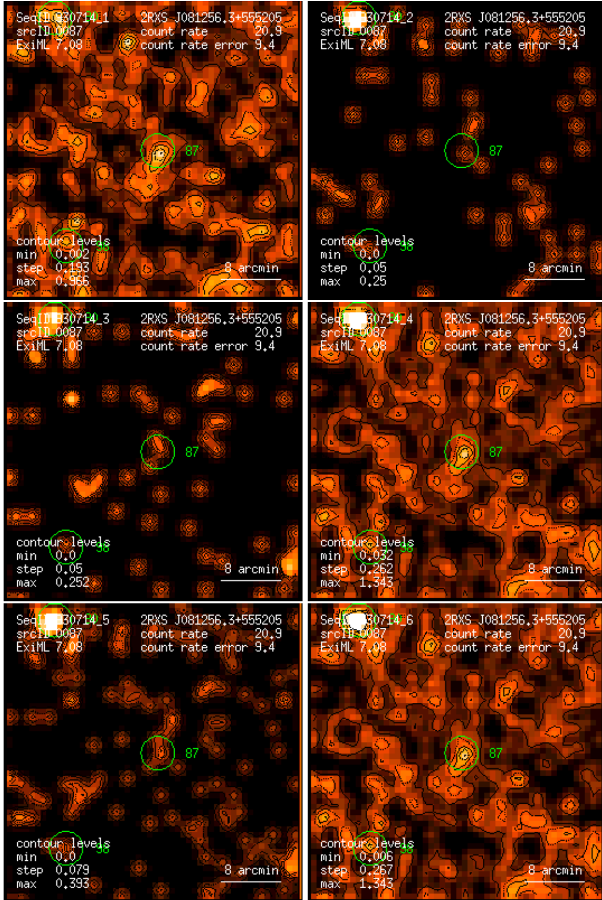
Figure 87: RASS 930714: detection 0087: band rate images, Gaussian filter: (1) PSPC channels 11 – 41, (2) 52 – 90, (3) 91 – 201, (4) 11 – 235, (5) 52 – 201, (6) 11 – 201. Broad band rates in counts/ks. Band rate contour levels in counts/ks/arcmin 2 .
