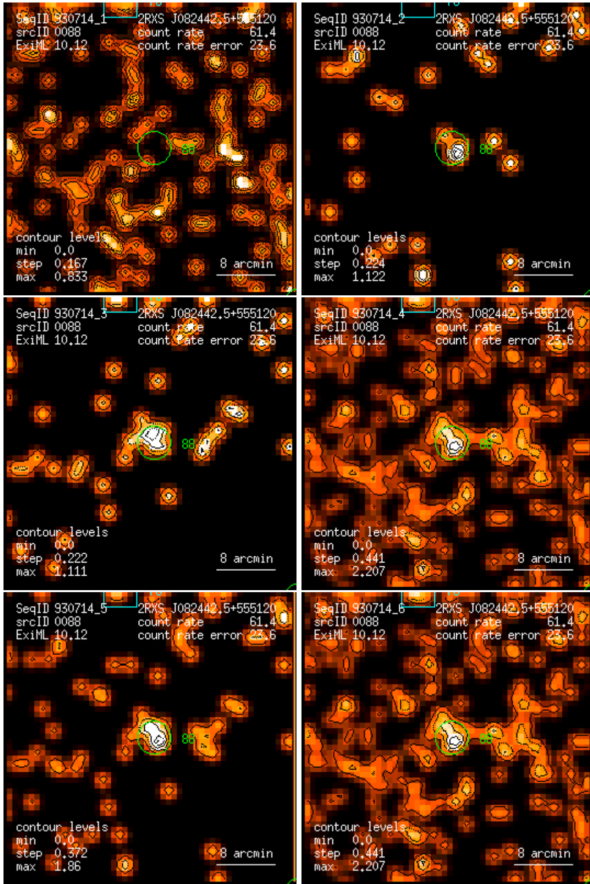
Figure 88: RASS 930714: detection 0088: band rate images, Gaussian filter: (1) PSPC channels 11 – 41, (2) 52 – 90, (3) 91 – 201, (4) 11 – 235, (5) 52 – 201, (6) 11 – 201. Broad band rates in counts/ks. Band rate contour levels in counts/ks/arcmin 2 .
