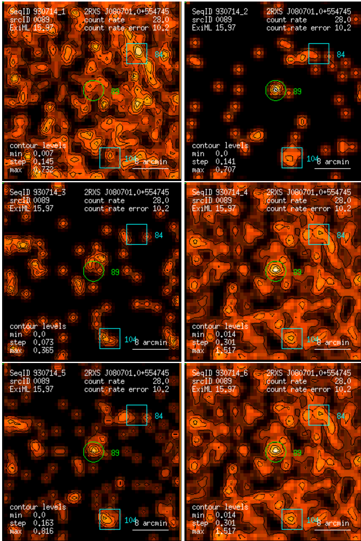
Figure 89: RASS 930714: detection 0089: band rate images, Gaussian filter: (1) PSPC channels 11 – 41, (2) 52 – 90, (3) 91 – 201, (4) 11 – 235, (5) 52 – 201, (6) 11 – 201. Broad band rates in counts/ks. Band rate contour levels in counts/ks/arcmin 2 .
